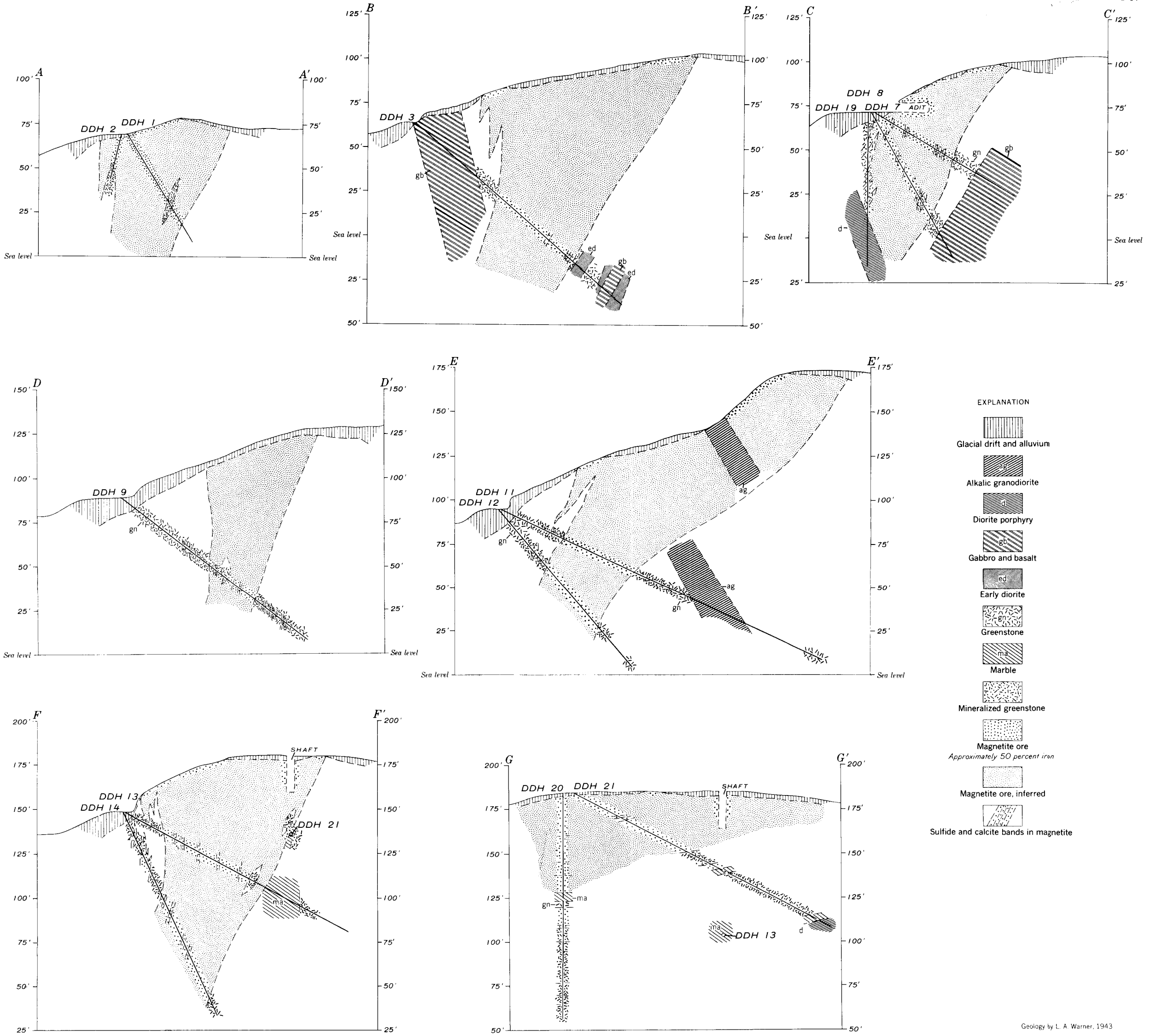
GEOLOGIC SECTIONS THROUGH DIAMOND-DRILL HOLES, POOR MAN IRON DEPOSIT
