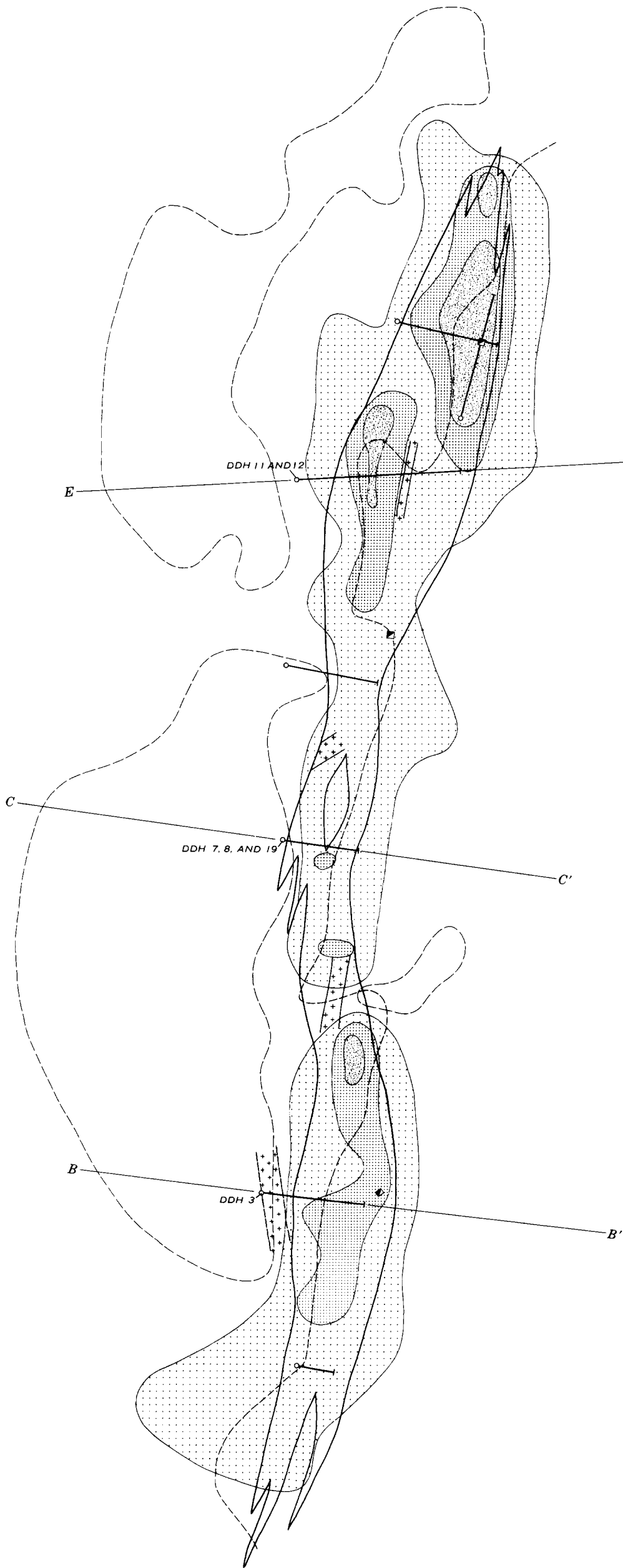
MAGNETIC MAP AND PROFILES, POOR MAN IRON DEPOSIT
