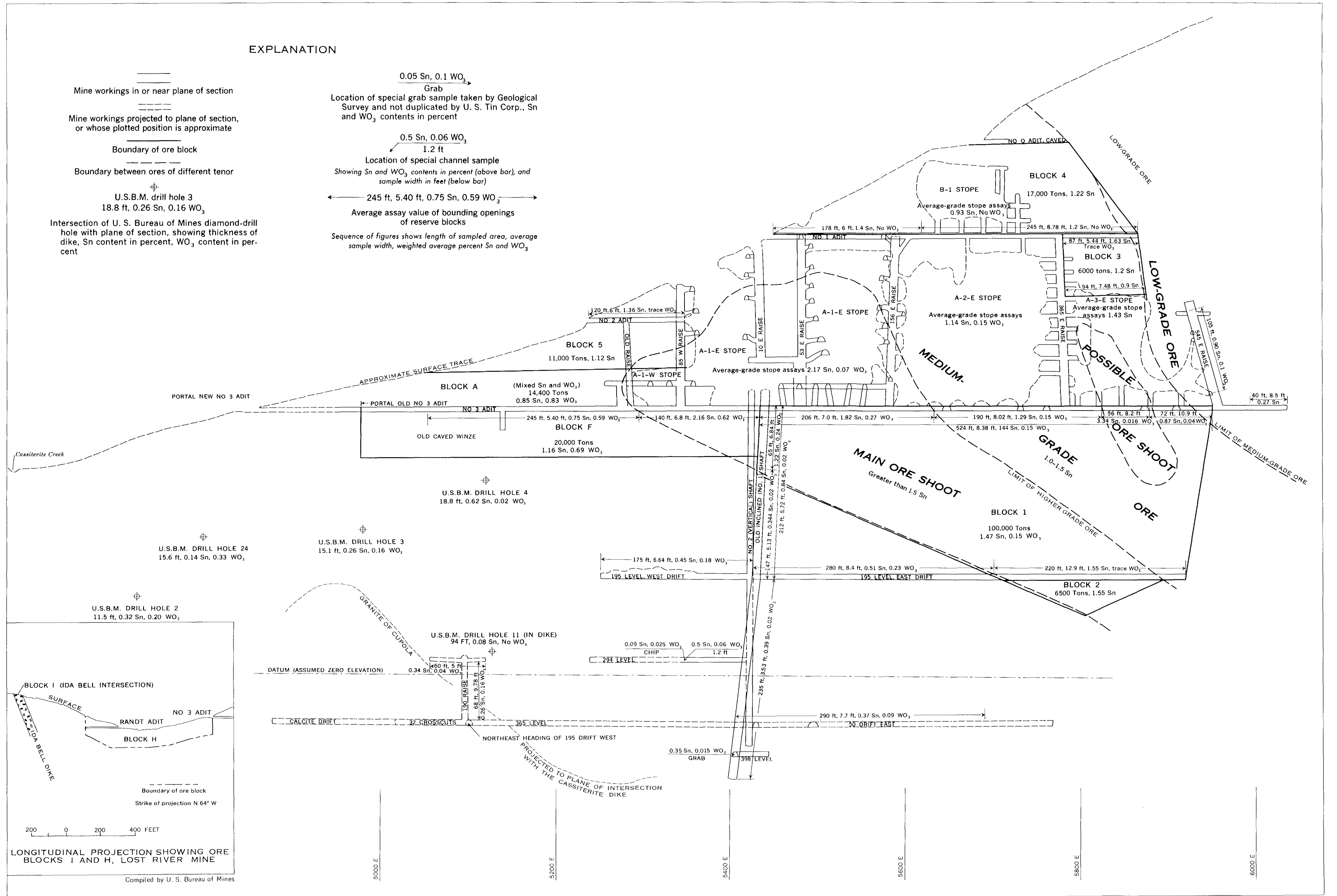
VERTICAL LONGITUDINAL PROJECTION SHOWING TIN ORE SHOOTS AND ORE RESERVE BLOCKS IN MAIN WORKINGS, LOST RIVER MINE, ALASKA
