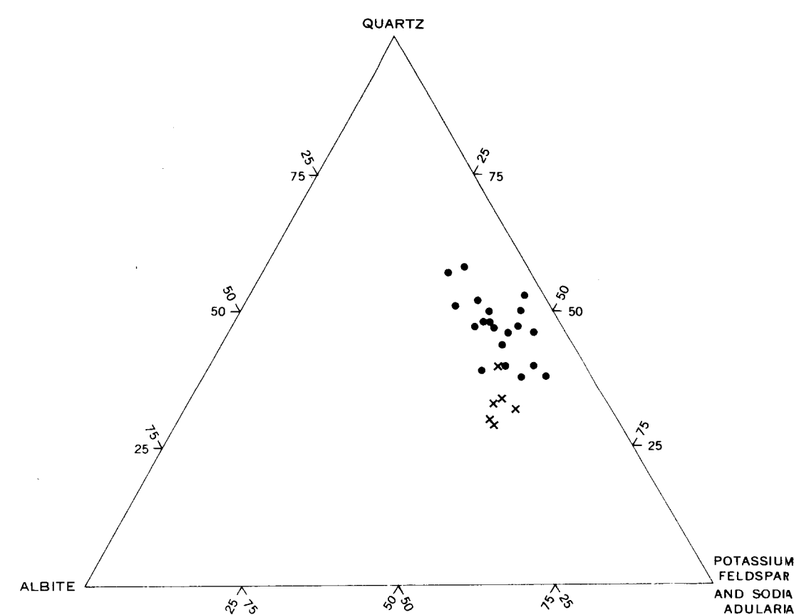
F. BOKAN MOUNTAIN GRANITE x Represents specimens from the Ross-Adams mine area
