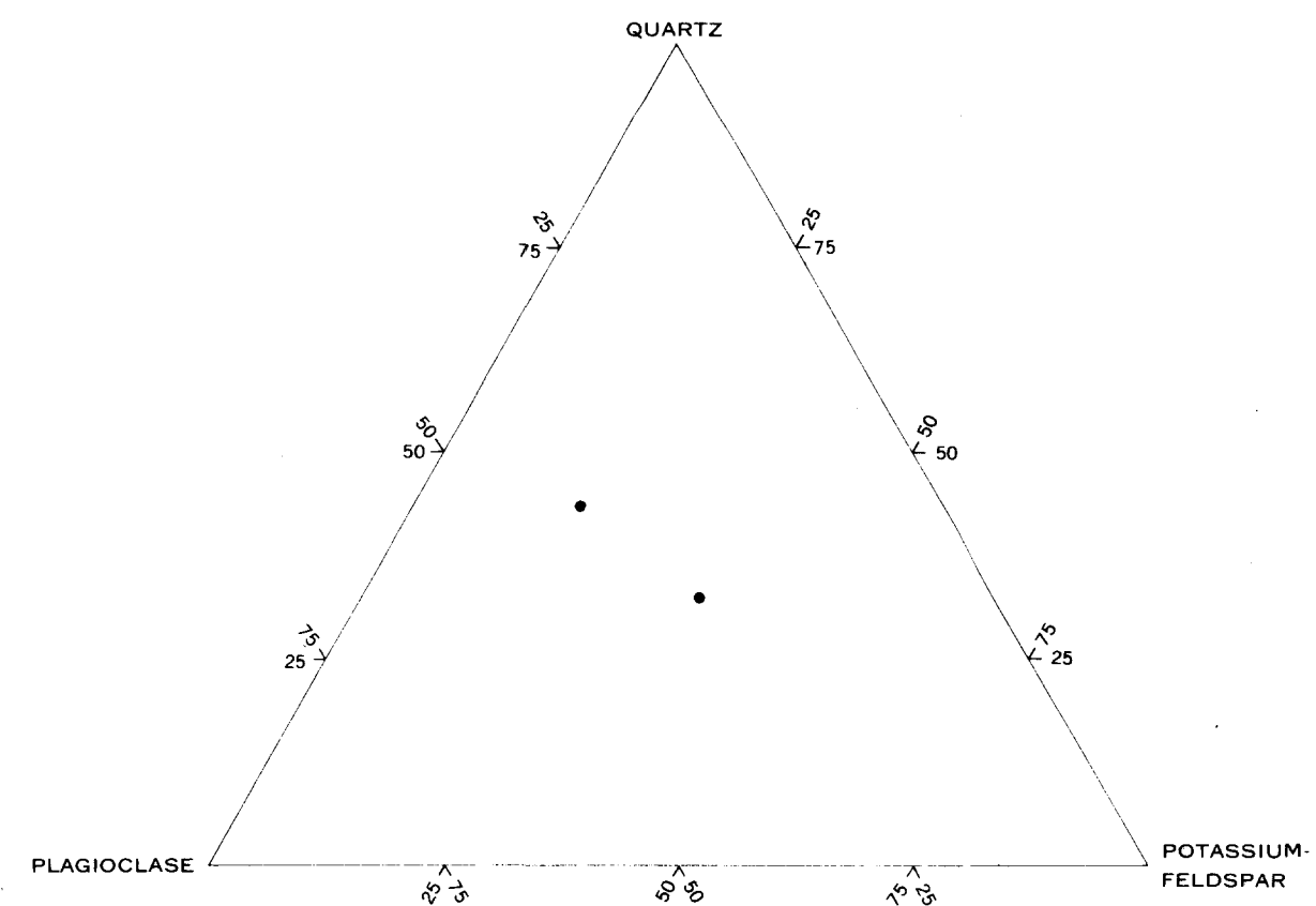
D. GNEISSIC QUARTZ MONZONITE
