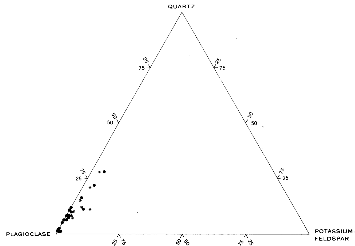
A. QUARTZ DIORITE AND DIORITE ● Albitized quartz diorite or diorite
