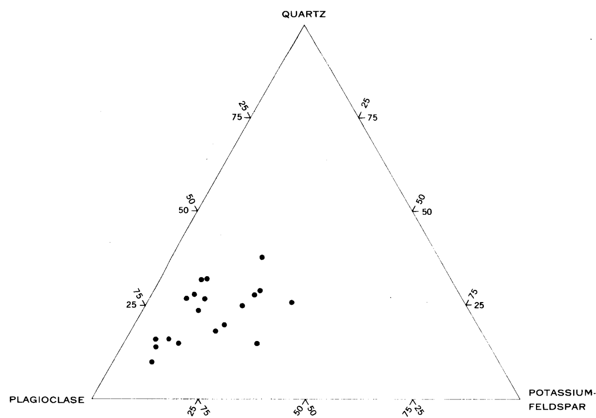
C. UNALBITIZED QUARTZ MONZONITE AND GRANODIORITE
