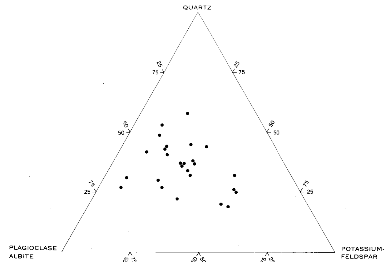
B. ALBITIZED QUARTZ MONZONITE AND GRANODIORITE
