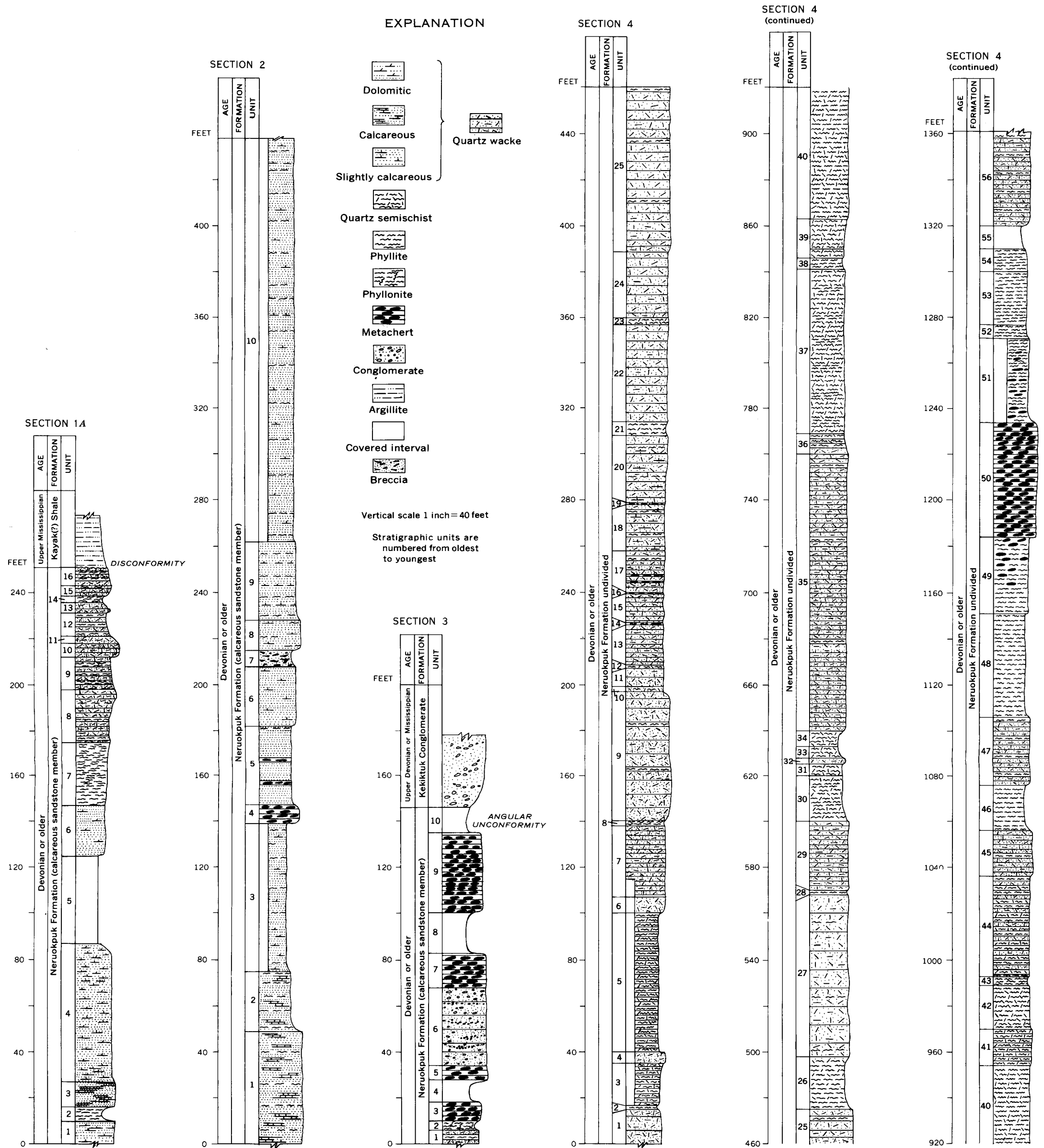
GRAPHIC SECTIONS OF THE NERUOKPUK FORMATION, LAKE PETERS AREA NORTHEASTERN BROOKS RANGE, ALASKA
