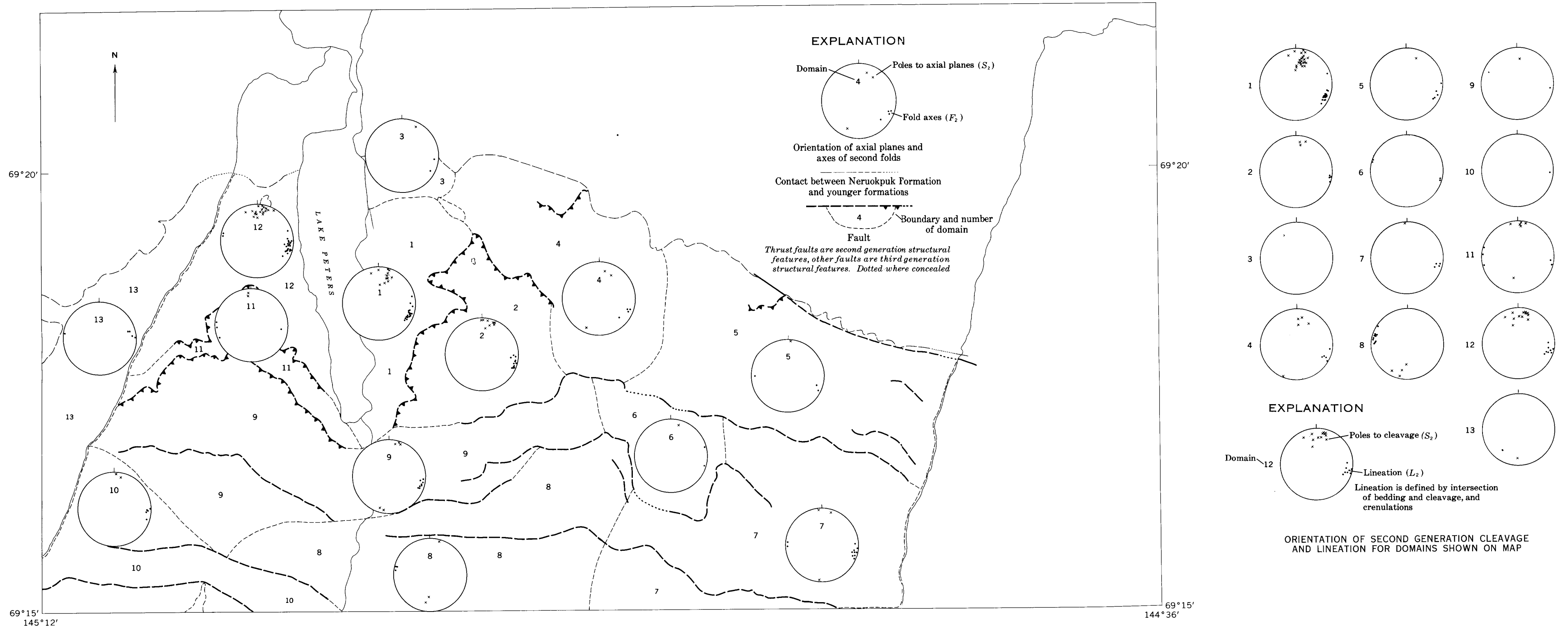
DIAGRAMS SHOWING ORIENTATION OF SECOND GENERATION STRUCTURAL FEATURES IN THE PETERS STRUCTURAL PROVINCE, ALASKA
