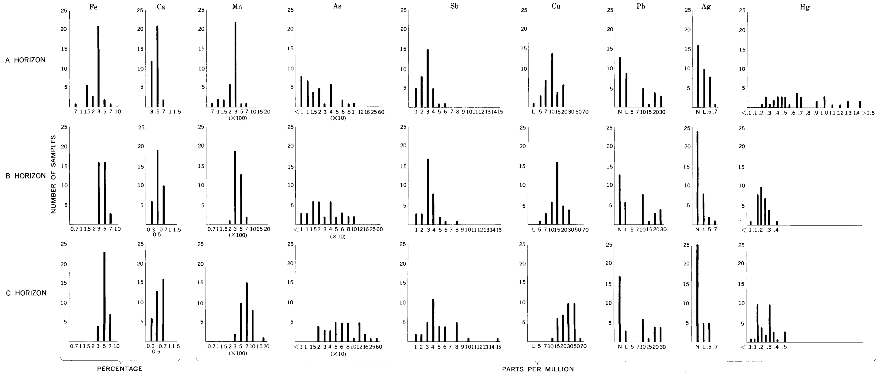
HISTOGRAMS SHOWING DISTRIBUTION OF IRON, CALCIUM, MANGANESE, ARSENIC, ANTIMONY, COPPER, LEAD, SILVER, AND MERCURY IN SOILS IN AREA B
