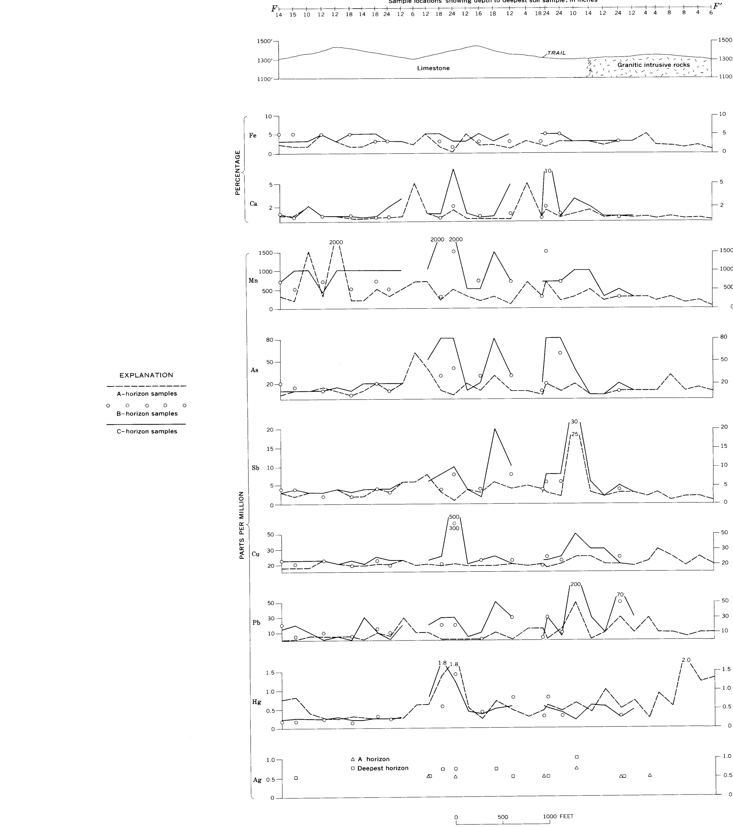
CONTENT AND DISTRIBUTION OF IRON, CALCIUM, MANGANESE, ARSENIC, ANTIMONY, COPPER, LEAD, MERCURY, SILVER, AND GOLD IN SOILS
