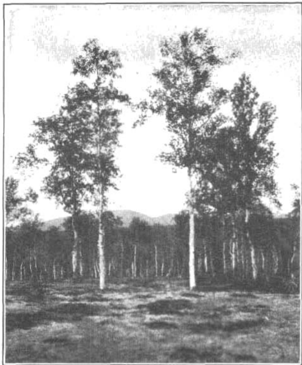
A. OPEN BIRCH FOREST ON HIGH, WELL-DRAINED SLOPES NEAR CAMP 27.
