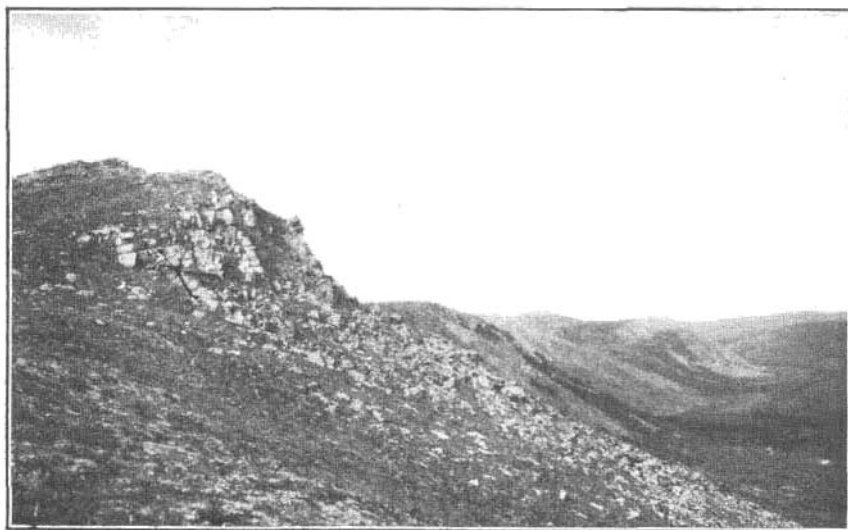
B. HOGBACK RIDGE SUPPORTED BY UPPER LIMB OF RECUMBENT SYNCLINAL FOLD.
