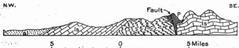
FIGURE 3.—Geologic cross section along line A-B on Plate II, near camp 33, showing unconformity and faulting between schist-quartzite group and Ordovician limestone. Lavas occur along the fault. ls, Ordovician limestone; sc, schist and quartzite; p, andesite porphyry; a, alluvium.
