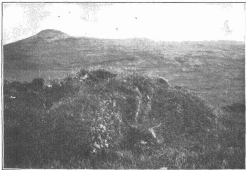
B. FOLDS IN TURF WHERE PART OF THE SLIDE CAME TO REST.
