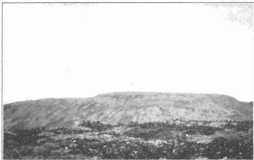
A. FLAT SUMMIT AND TERRACES DUE TO ALTIPLANATION, GRANITE MOUNTAIN 2 MILES SOUTH-WEST OF CAMP 24.
