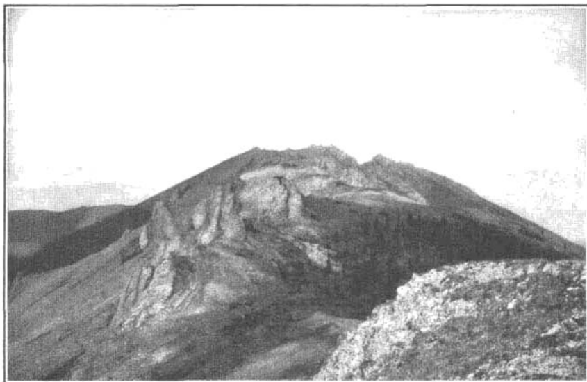
A. THIN-BEDDED ORDOVICIAN LIMESTONES UNDERLYING FOSSILIFEROUS MEMBER, LOOKING NORTHEAST FROM FOSSIL LOCALITY 1 MILE NORTHWEST OF CAMP 36.
