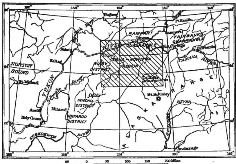
FIGURE 1.—Index map showing relation of the Cosna-Nowitna region to other districts of interior Alaska.
