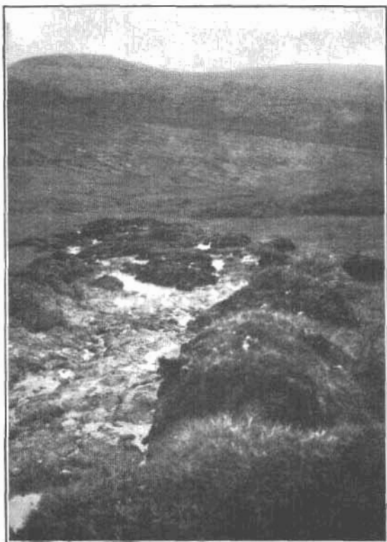
A. VIEW LOOKING DOWN THE COURSE OF A RECENT LANDSLIDE IN THE UPLANDS BETWEEN CAMPS 12 AND 13.
