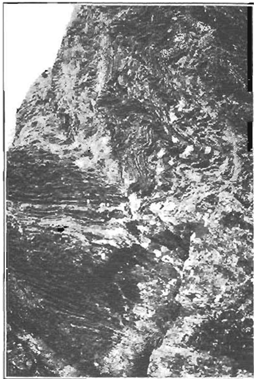
X. CHERTY PRE-ORDOVICIAN LIMESTONE 2 MILES NORTH- EAST OF CAMP 41.
