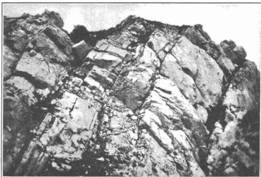
B. MASSIVE ORDOVICIAN LIMESTONES 1,500 FEET BELOW FOSSIL HORIZON, 3 MILES NORTH OF CAMP 36.
