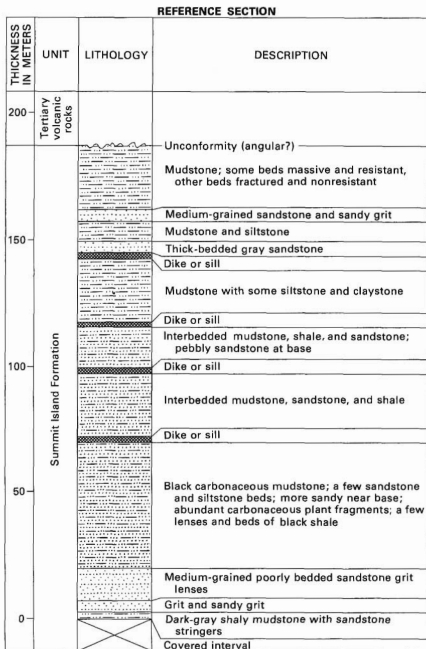
FIGURE 7.—Sections of the Upper Cretaceous Summit Island Formation in southwestern Alaska. Location of sections shown on figure 1.
