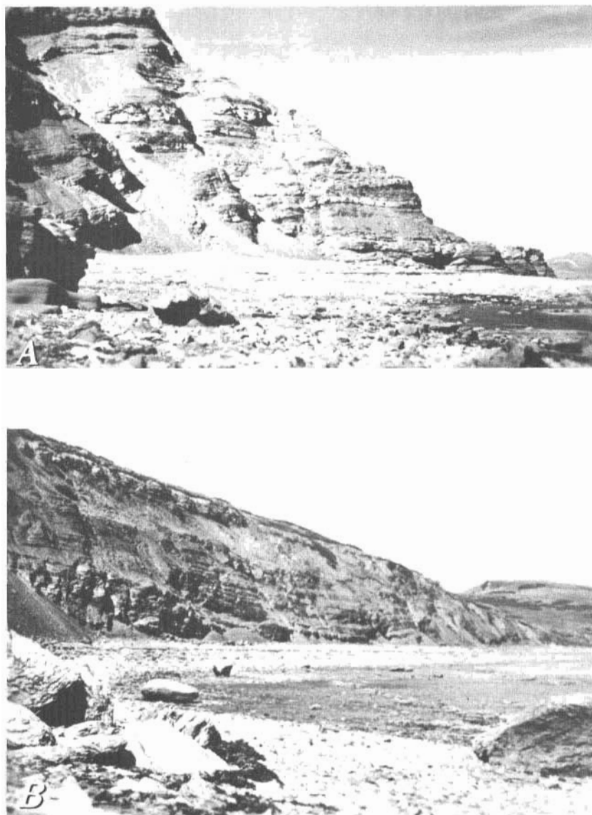
FIGURE 5.—Carbonaceous mudstone, siltstone, shale, and sandstone in reference section of Summit Island Formation on east side of unnamed headland on mainland, 6 km northeast of Summit Island (figs. 1, 2). A , North view of nearly flat lying Summit Island Formation exposed in central part of reference section. B , Sea-cliff exposures at north end of reference section. Plant fossils occur at base of cliff near center of photograph. Boulders in foreground from a large rhyolite sill. Beds dip eastward; view north.
