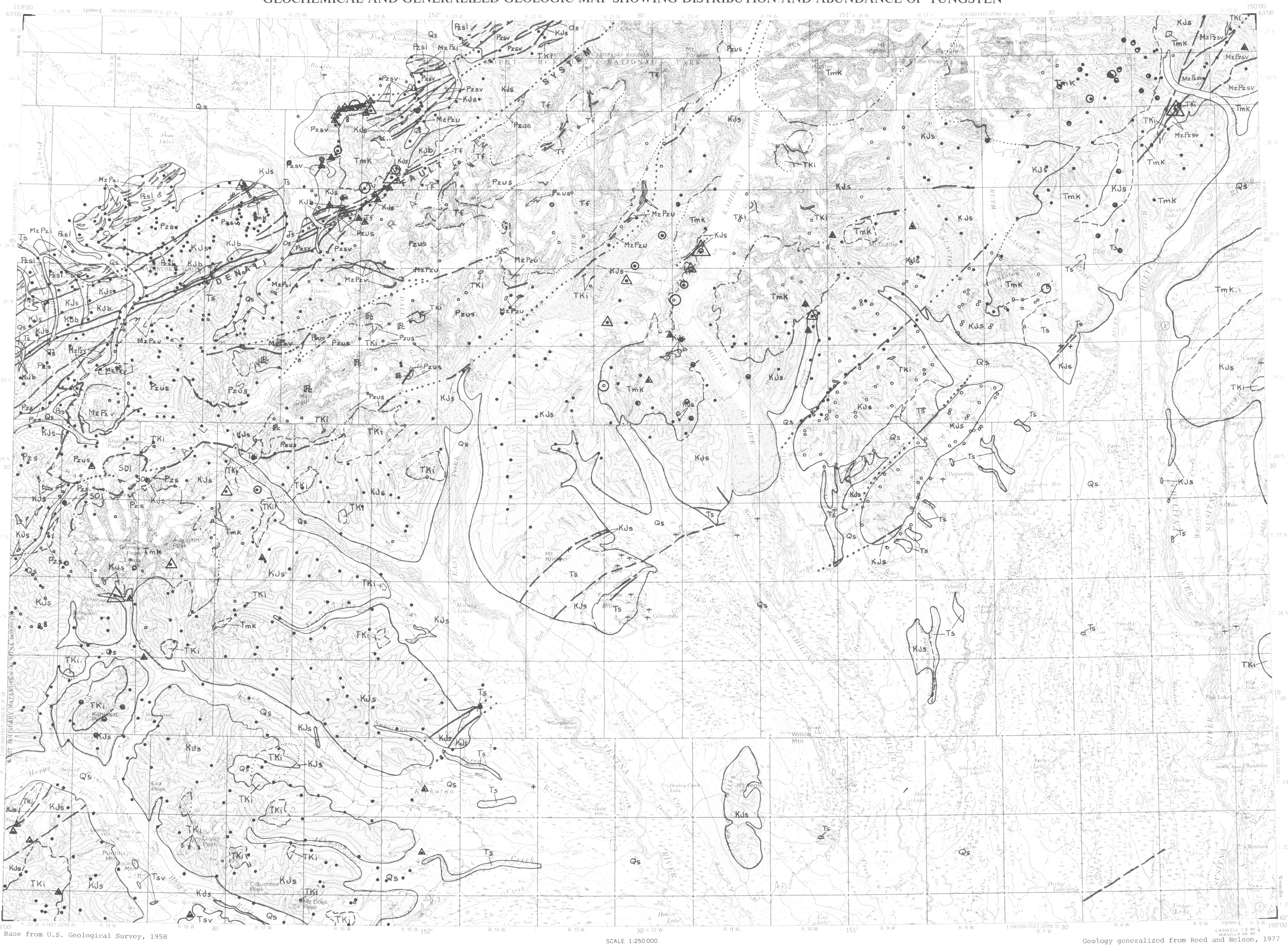
GEOCHEMICAL AND GENERALIZED GEOLOGIC MAP SHOWING DISTRIBUTION AND ABUNDANCE OF TUNGSTEN
