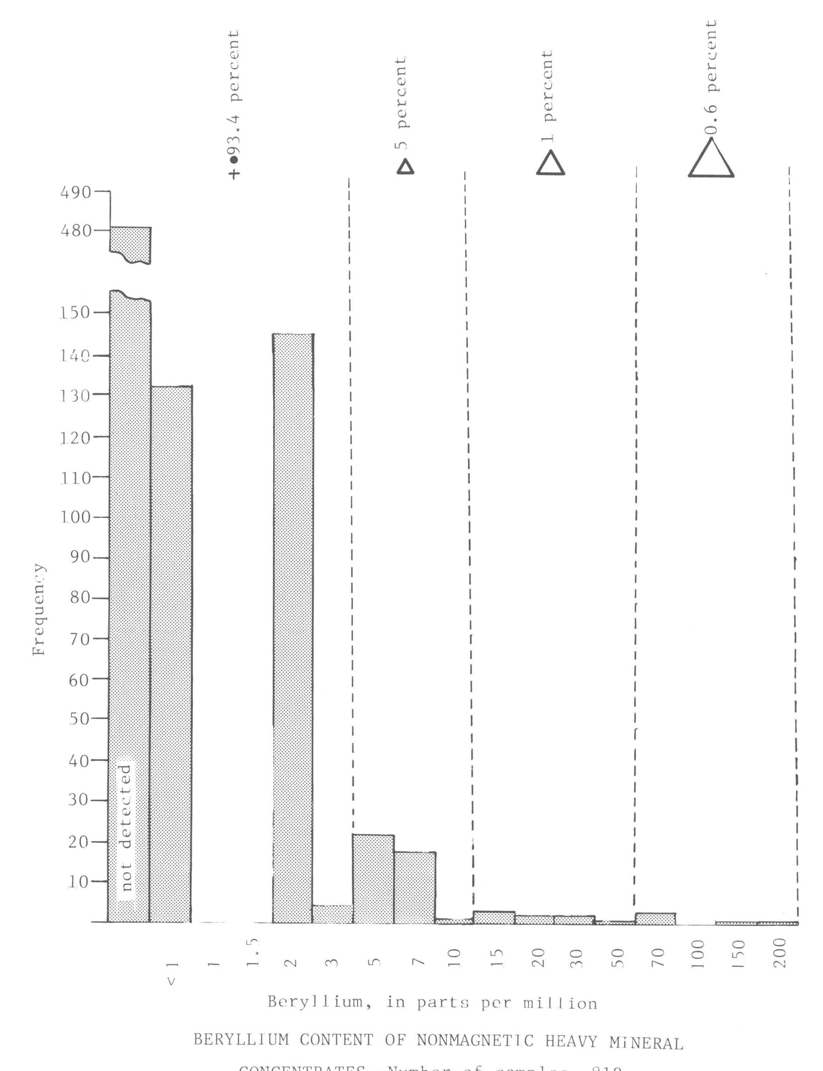
Beryllium, in parts per million BERYLLIUM CONTENT OF NONMAGNETIC HEAVY MINERAL CONCENTRATES--Number of samples, 819.
