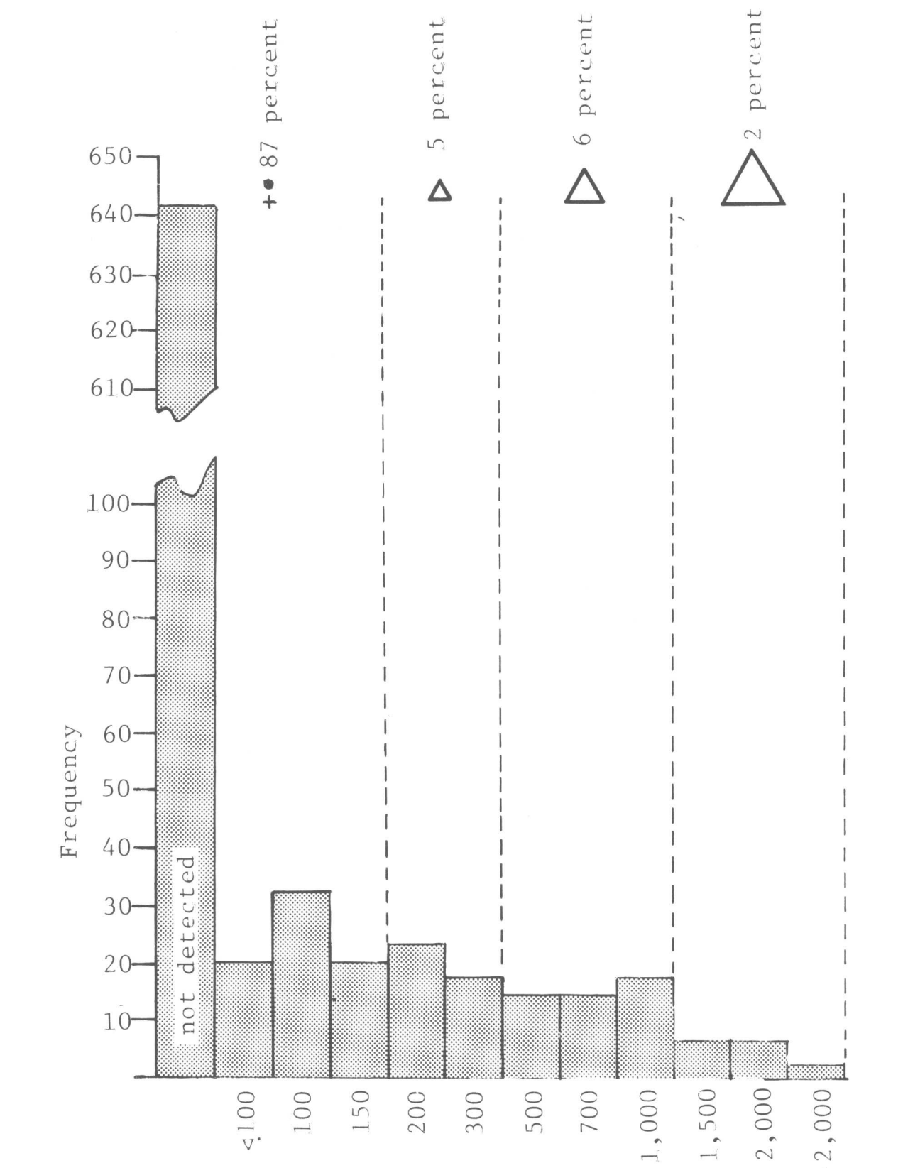
Tungsten, in parts per million TUNGSTEN CONTENT OF NONMAGNETIC HEAVY MINERAL CONCENTRATES--Number of samples, 819.
