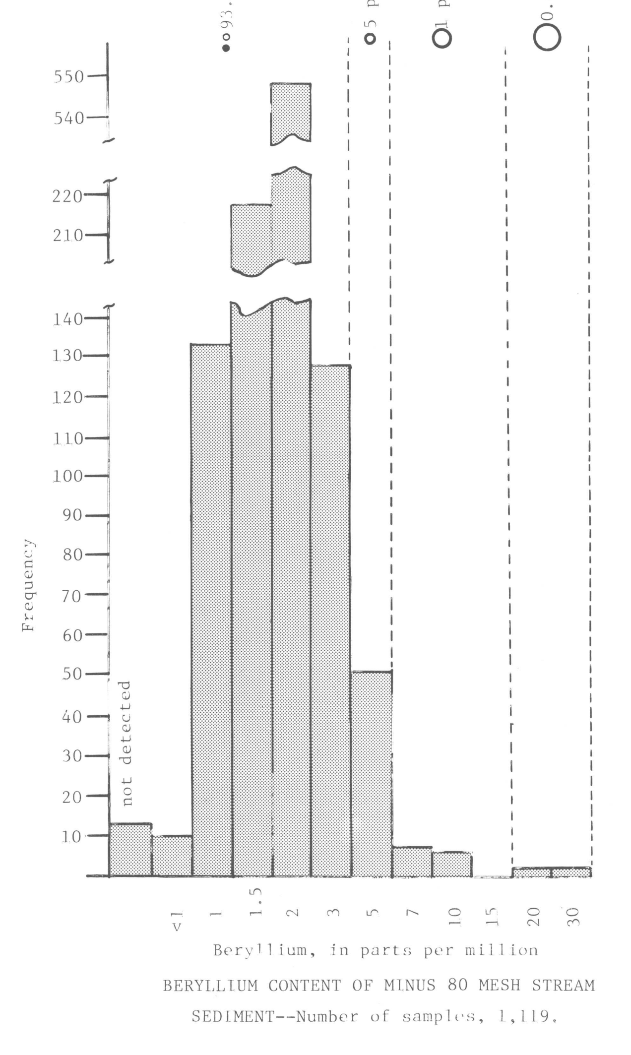
Beryllium, in parts per million BERYLLIUM CONTENT OF MINUS 80 MESH STREAM SEDIMENT--Number of samples, 1,119.
