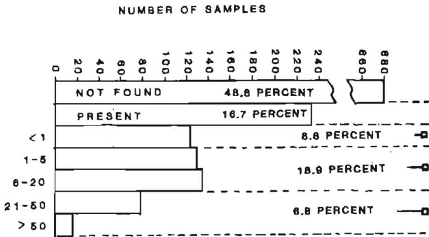
PYRITE CONTENT IN PERCENT
