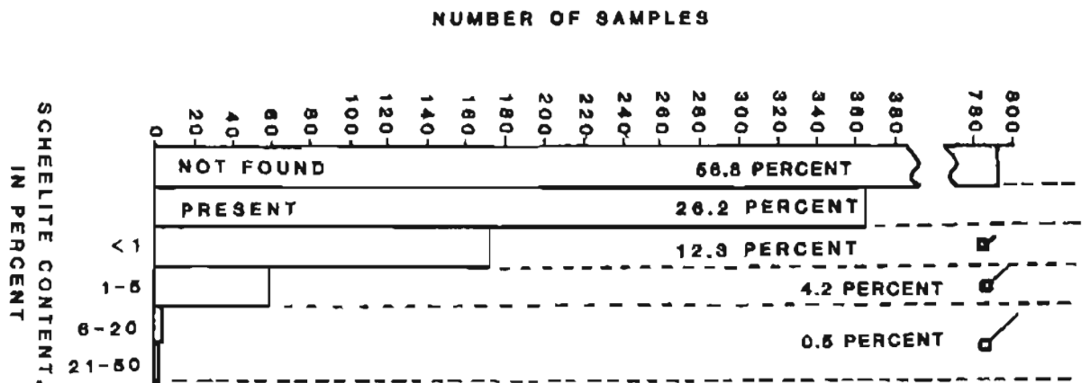
Figure 2.—Histograms showing amounts of cassiterite, gold, and scheelite in nonmagnetic heavy-mineral-concentrate samples from stream sediment, Solomon and Bendeleben 1° x 3° quadrangles. Symbols (star-diagram rays), which vary in length to denote amounts of minerals present, correspond to symbols used on map B
