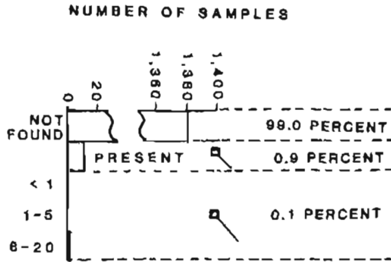
GALENA CONTENT, IN PERCENT
