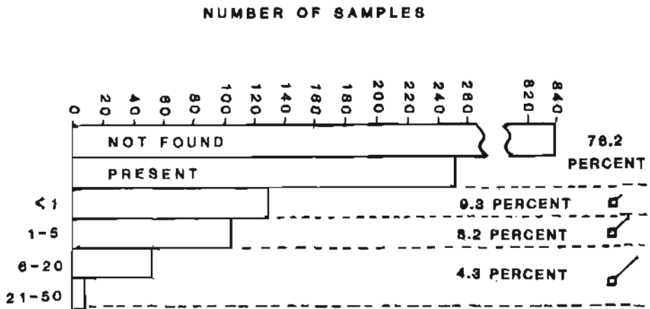
TOURMALINE CONTENT, IN PERCENT
