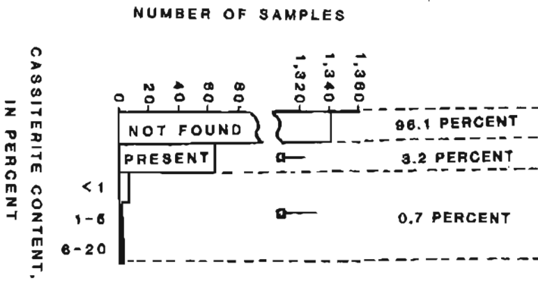
Figure 2.—Histograms showing amounts of cassiterite, gold, and scheelite in nonmagnetic heavy-mineral-concentrate samples from stream sediment, Solomon and Bendeleben 1° x 3° quadrangles. Symbols (star-diagram rays), which vary in length to denote amounts of minerals present, correspond to symbols used on map B
