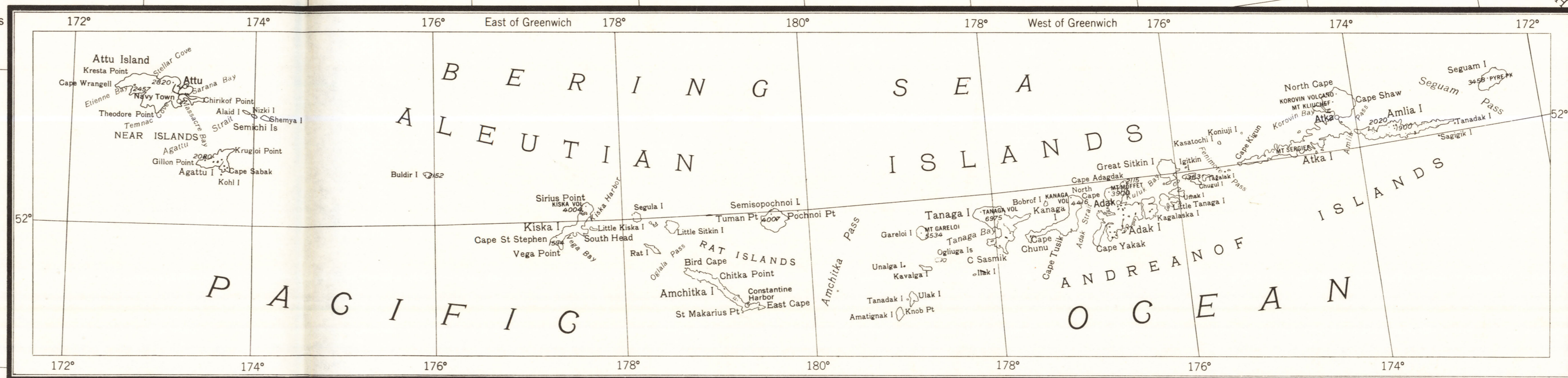
TUNGSTEN OCCURRENCES IN ALASKA Compiled by Edward H. Cobb 1975
