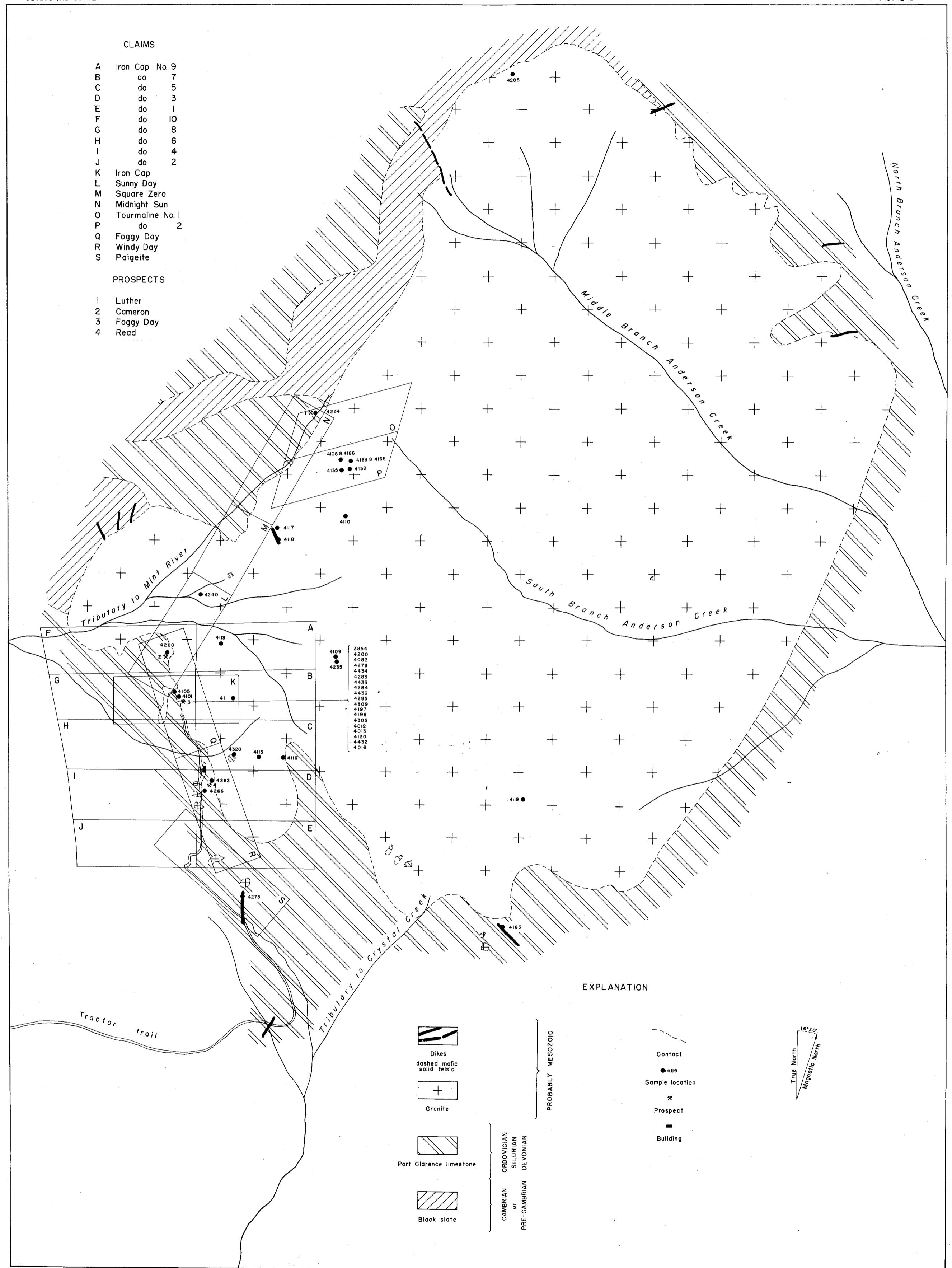
GEOLOGIC MAP OF THE BROOKS MOUNTAIN AREA, TELLER QUADRANGLE, SEWARD PENINSULA, ALASKA
