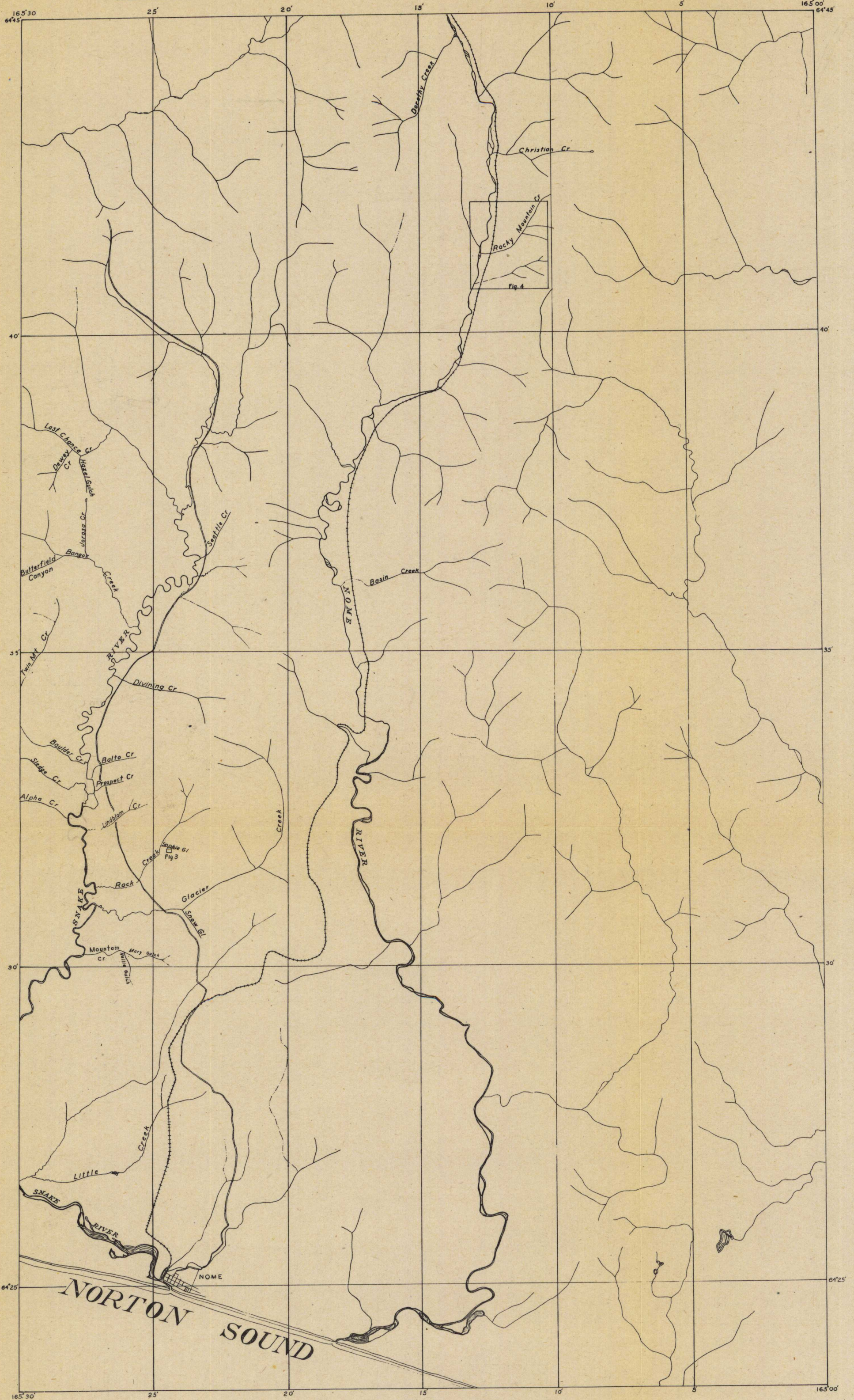
Figure 2 MAP OF THE NOME AREA, SHOWING LOCATION OF STREAMS FROM PLACERS OF WHICH SCHEELITE HAS BEEN REPORTED AND AREAS OF KNOWN LODE SCHEELITE DEPOSITS
