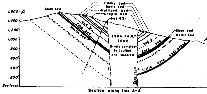
FIGURE 4 GEOLOGIC STRUCTURE SECTIONS ACROSS THE EASTERN PART OF THE LOWER MATANUSKA VALLEY COAL FIELD, ALASKA
