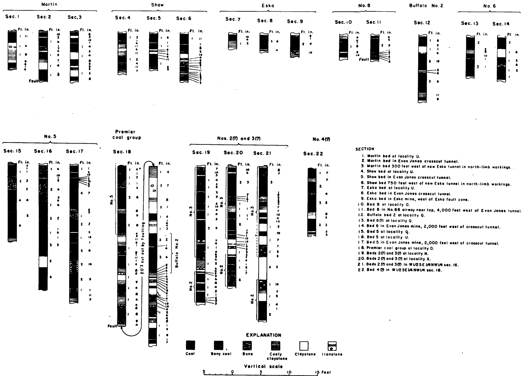
Figure 5.— Sections of coal beds in eastern part of lower Matanuska Valley coal field.
