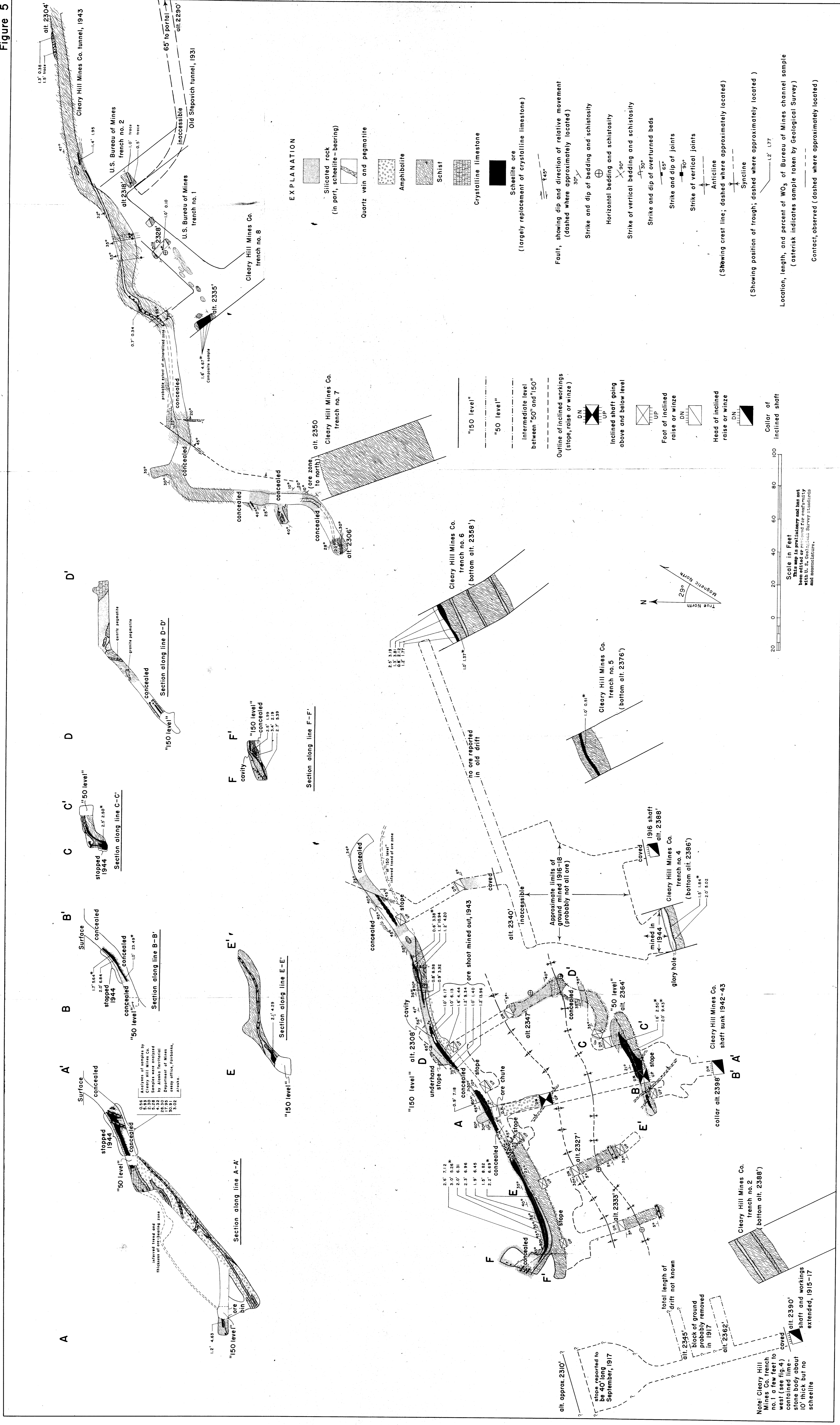
GEOLOGIC MAP AND SECTIONS OF STEPOVICH MINE
