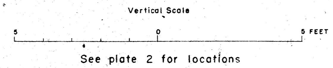
DETAILED SECTIONS OF COAL BEDS IN THE SOUTHERN PART OF THE HOMER DISTRICT
