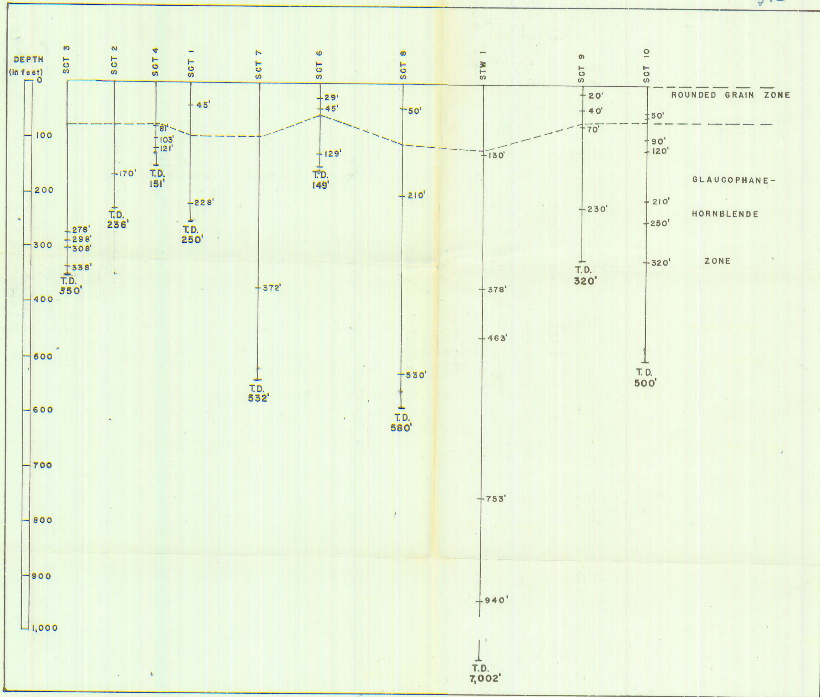
FIGURE 3. CORRELATION OF SIMPSON TEST WELL NO. 1 AND SIMPSON CORE TESTS NOS. 1-4, 6-10 BY HEAVY MINERAL ZONES
