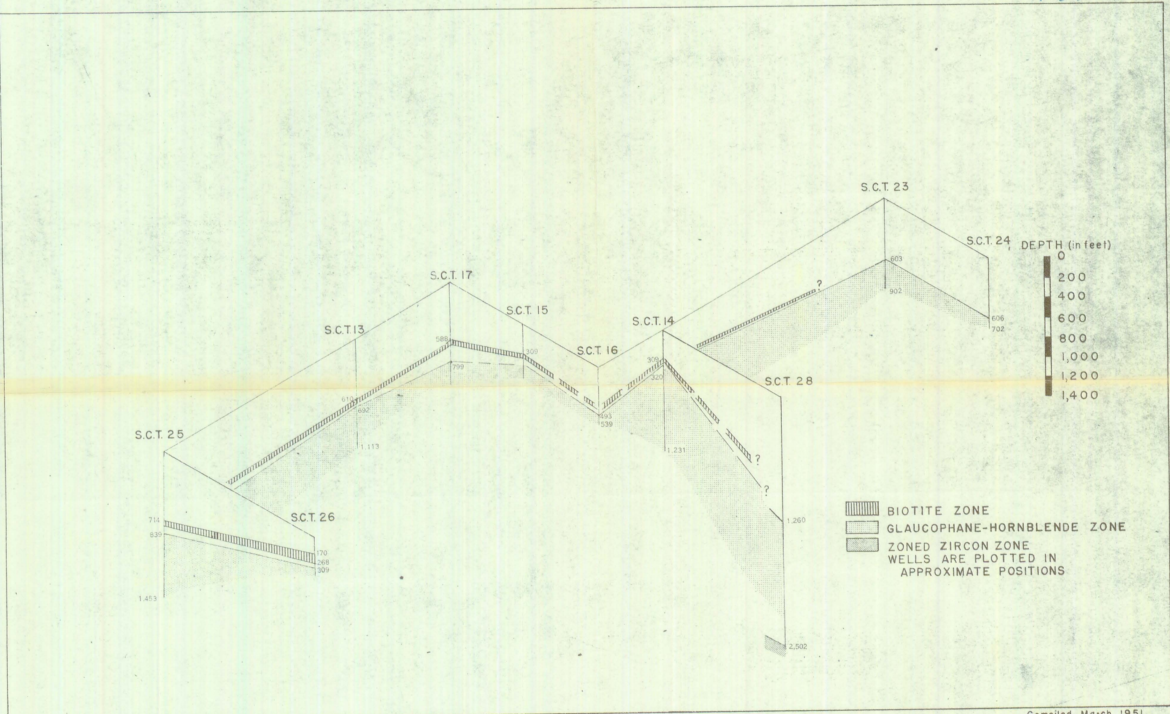
FIGURE 4. CORRELATION OF SIMPSON CORE TESTS NOS. 13-17, 23-26, AND 28 BY HEAVY MINERAL ZONES
