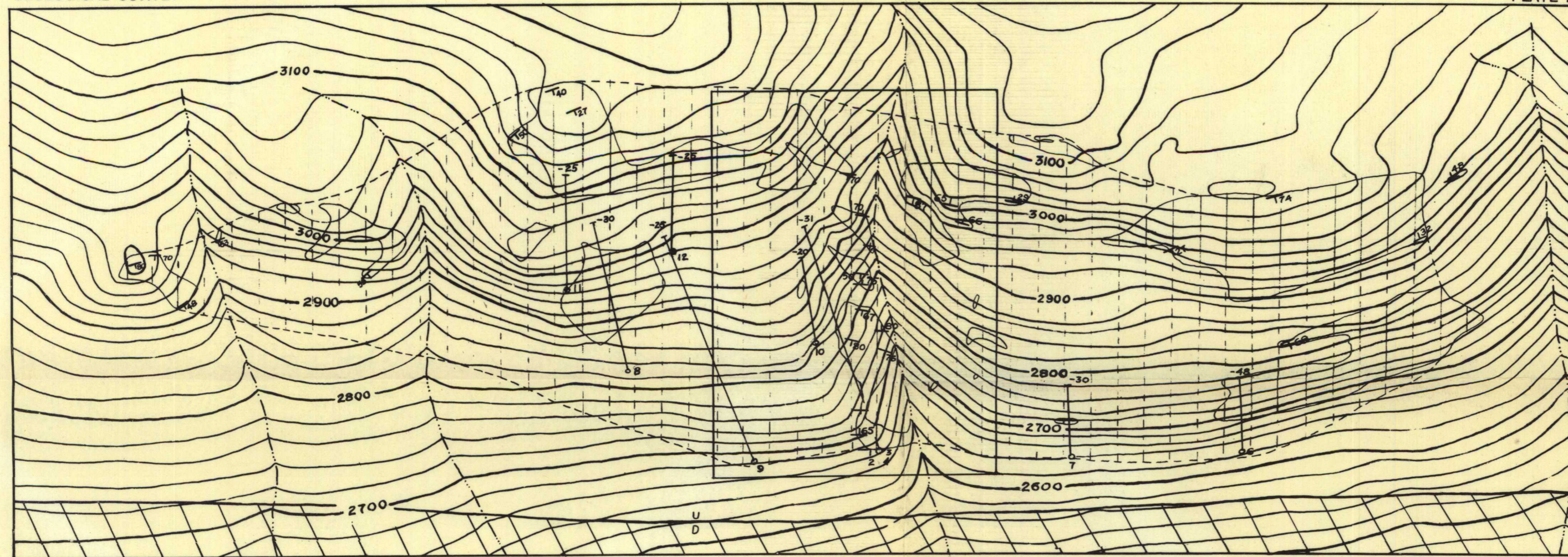
Geology by E.H. Cobb, 1947 with additions by R.M. Moxham and R.A. Eckhart, 1951.
