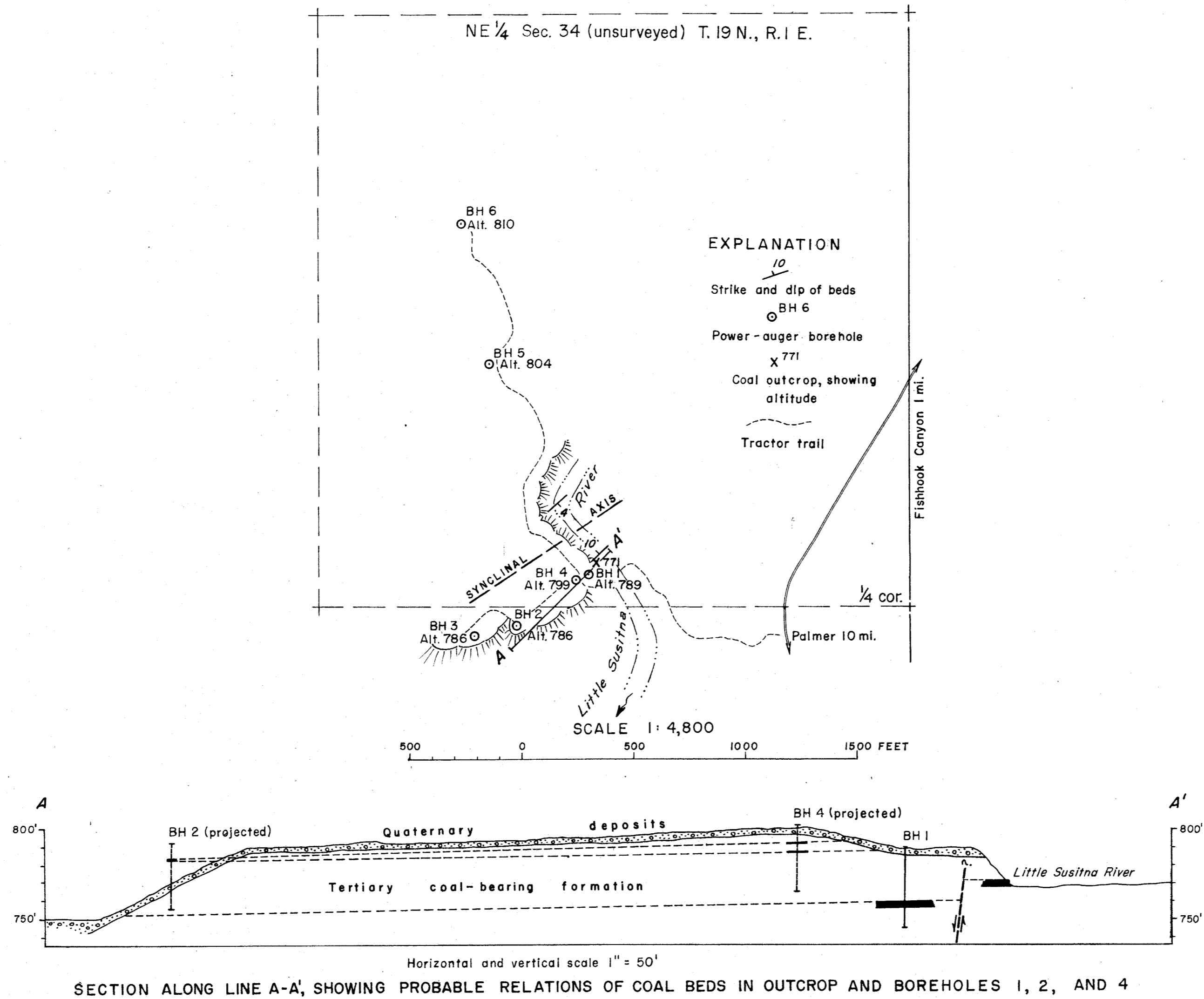
SKETCH MAP AND SECTION OF LOCALITY 6, LITTLE SUSITNA DISTRICT, MATANUSKA COAL FIELD, ALASKA
