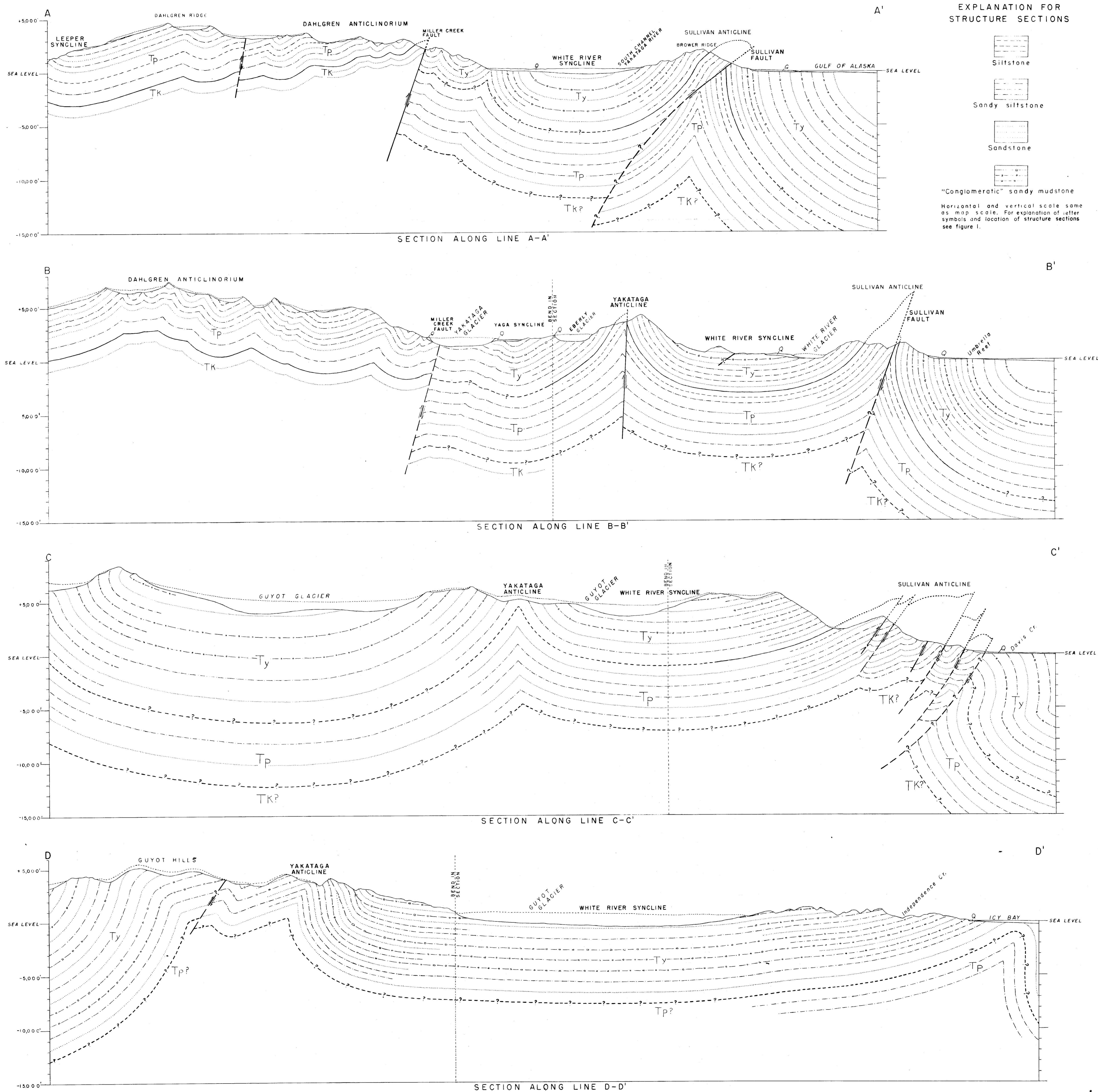
STRUCTURE SECTIONS OF THE SOUTHEASTERN PART OF THE ROBINSON MOUNTAINS, YAKATAGA DISTRICT, ALASKA
