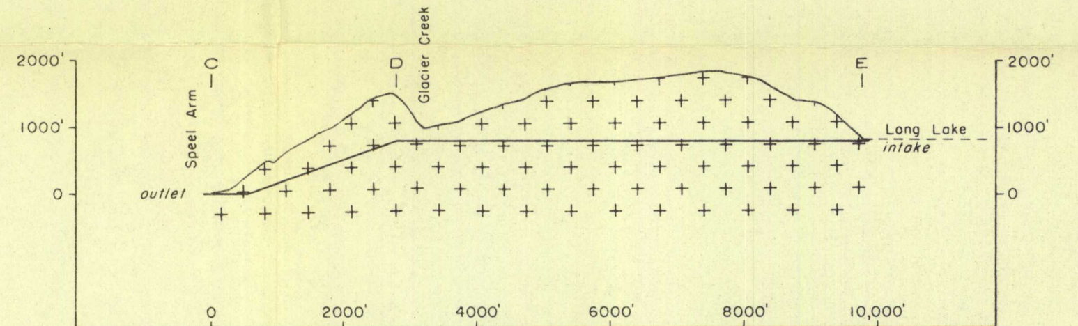
Section along line C-D-E (see plate 3)
