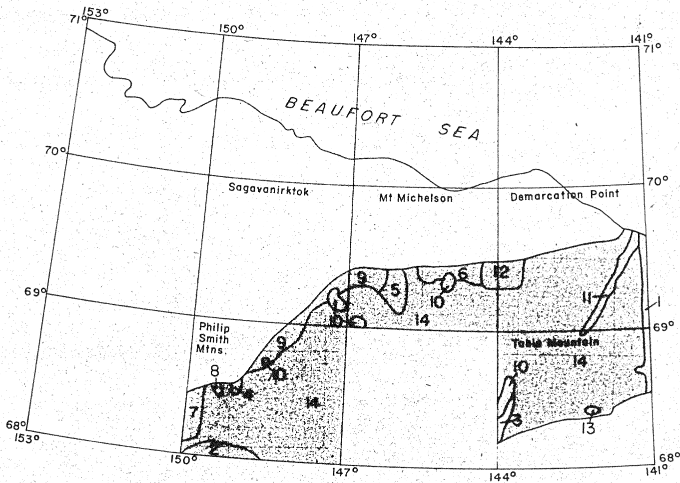
Index map showing location of area and sources of geologic data.
