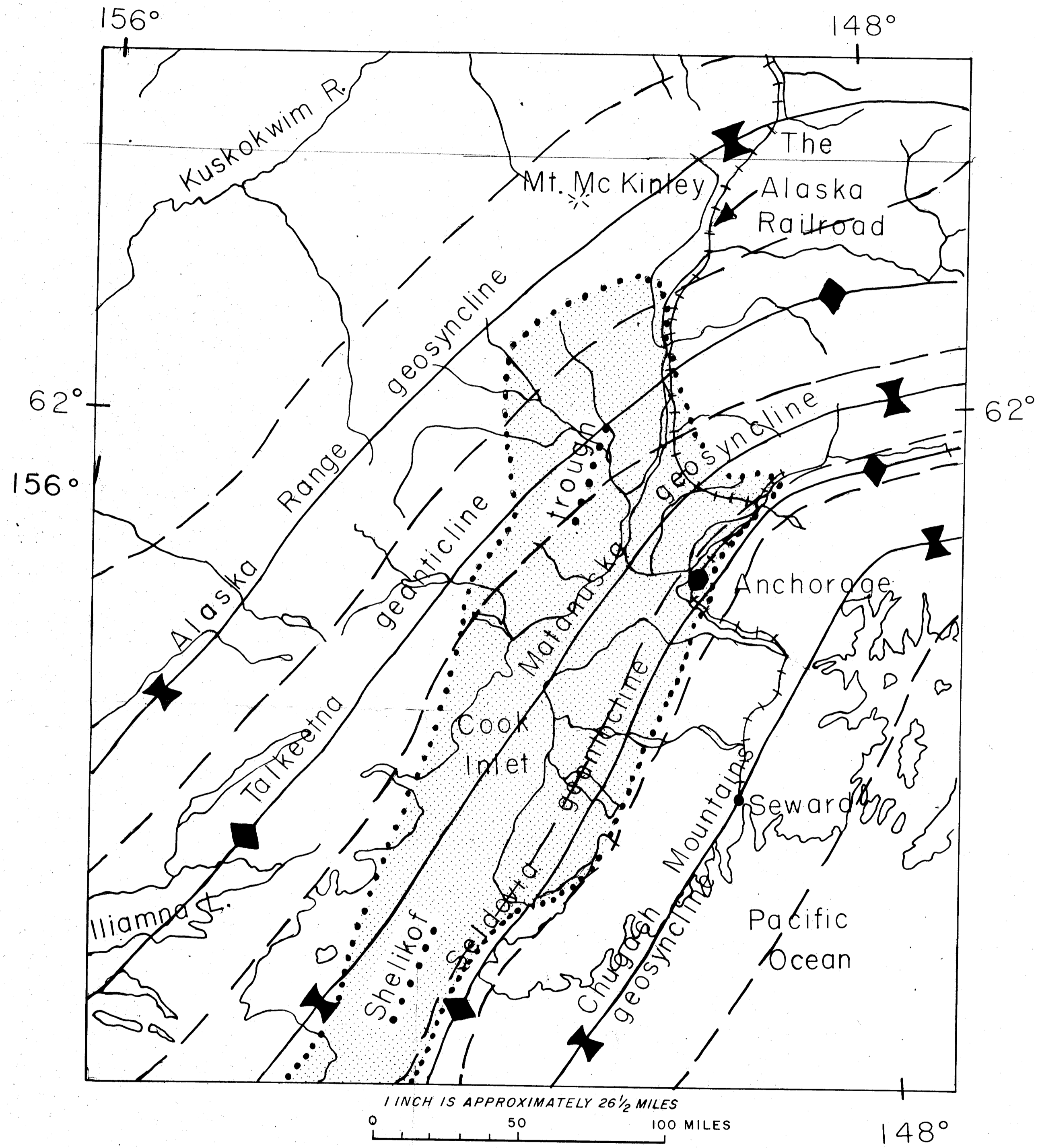
Figure 7. Outline of the Mesozoic and Cenozoic tectonic elements of the Cook Inlet area, Alaska. (After Payne, 1955)
