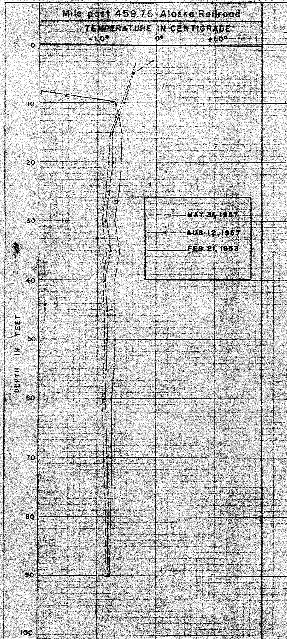
Fig. 11.--Thermal profiles of permafrost near Fairbanks, Alaska
