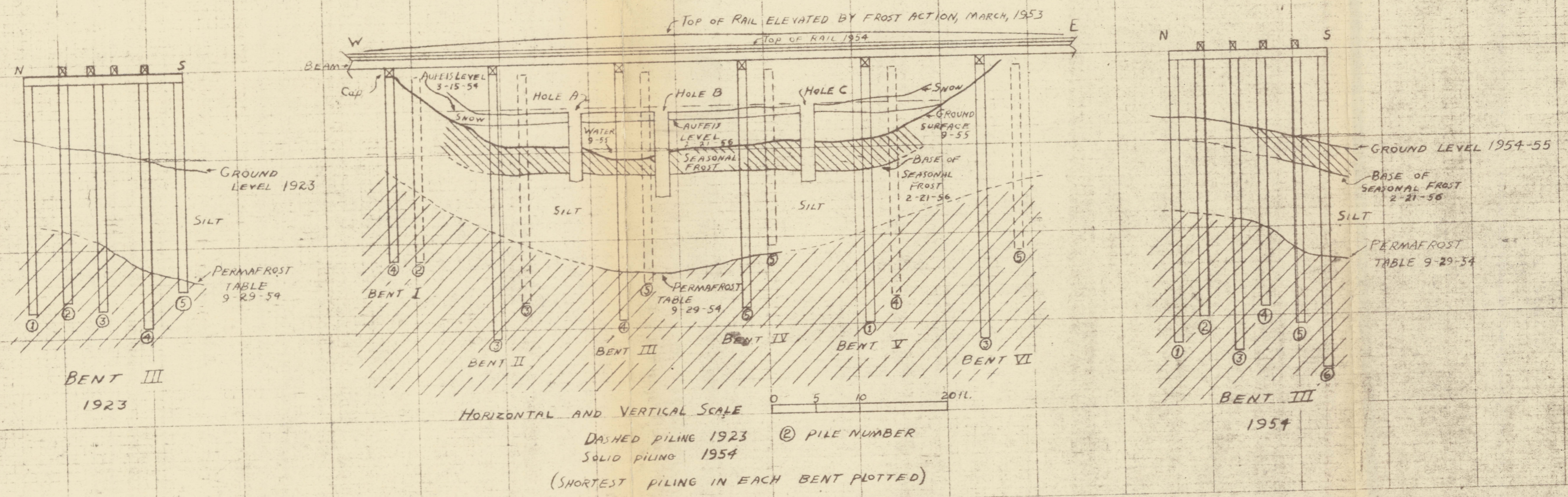
Fig. 22.--Geologic cross sections at bridge at Mile Post 458.4 in Goldstream Valley, Fairbanks, Alaska The Alaska Railroad
