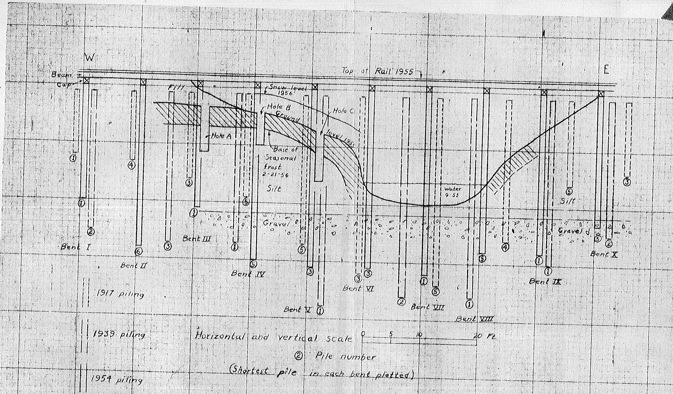
Fig. 25.--Geologic cross section at bridge at Mile Post 460.4 over Goldstream Creek near Fairbanks, Alaska
