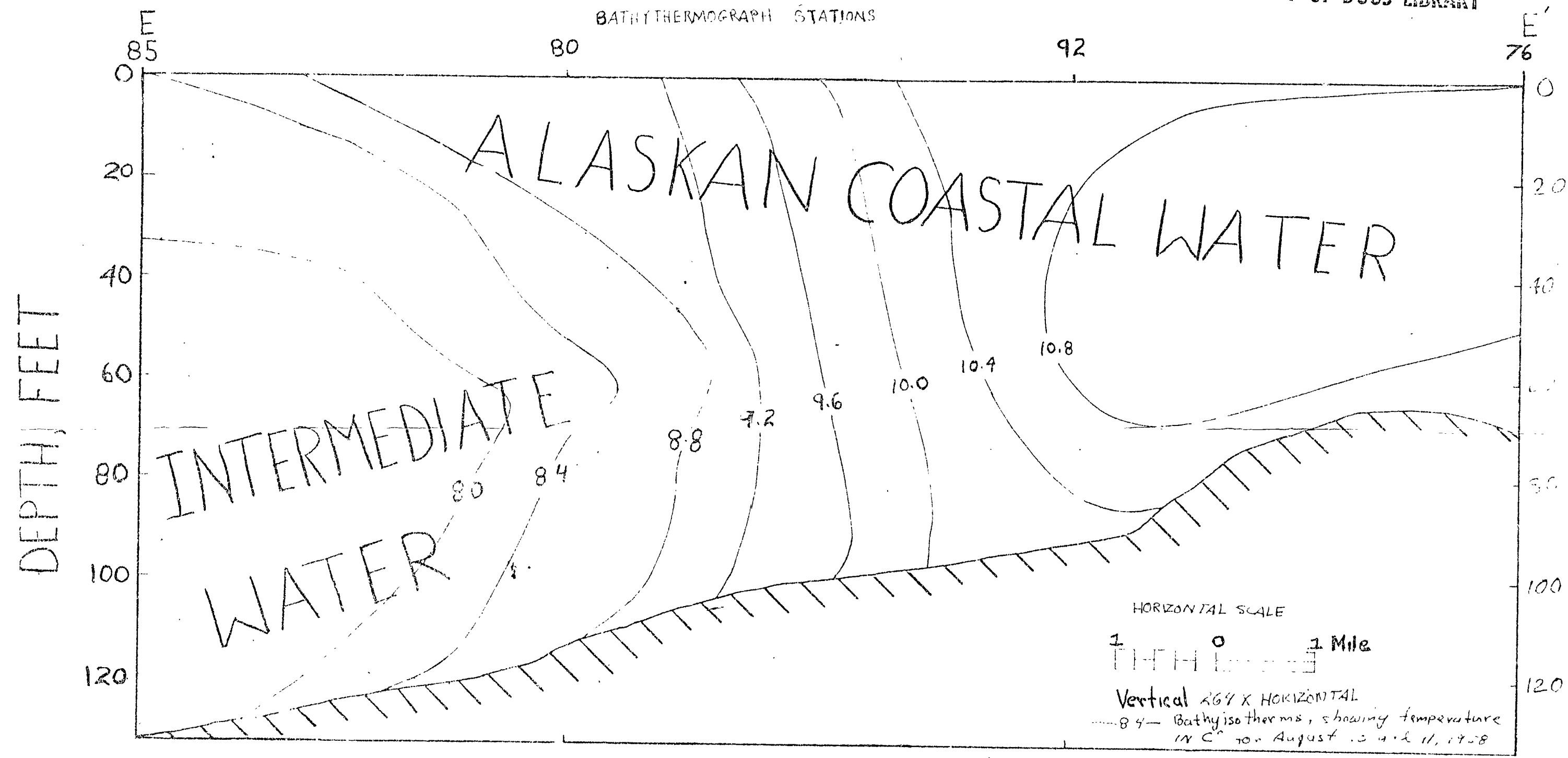
Figure 5 Vertical temperature section E-E'; positions of bathythermograph stations and section line are shown on figure 2.
