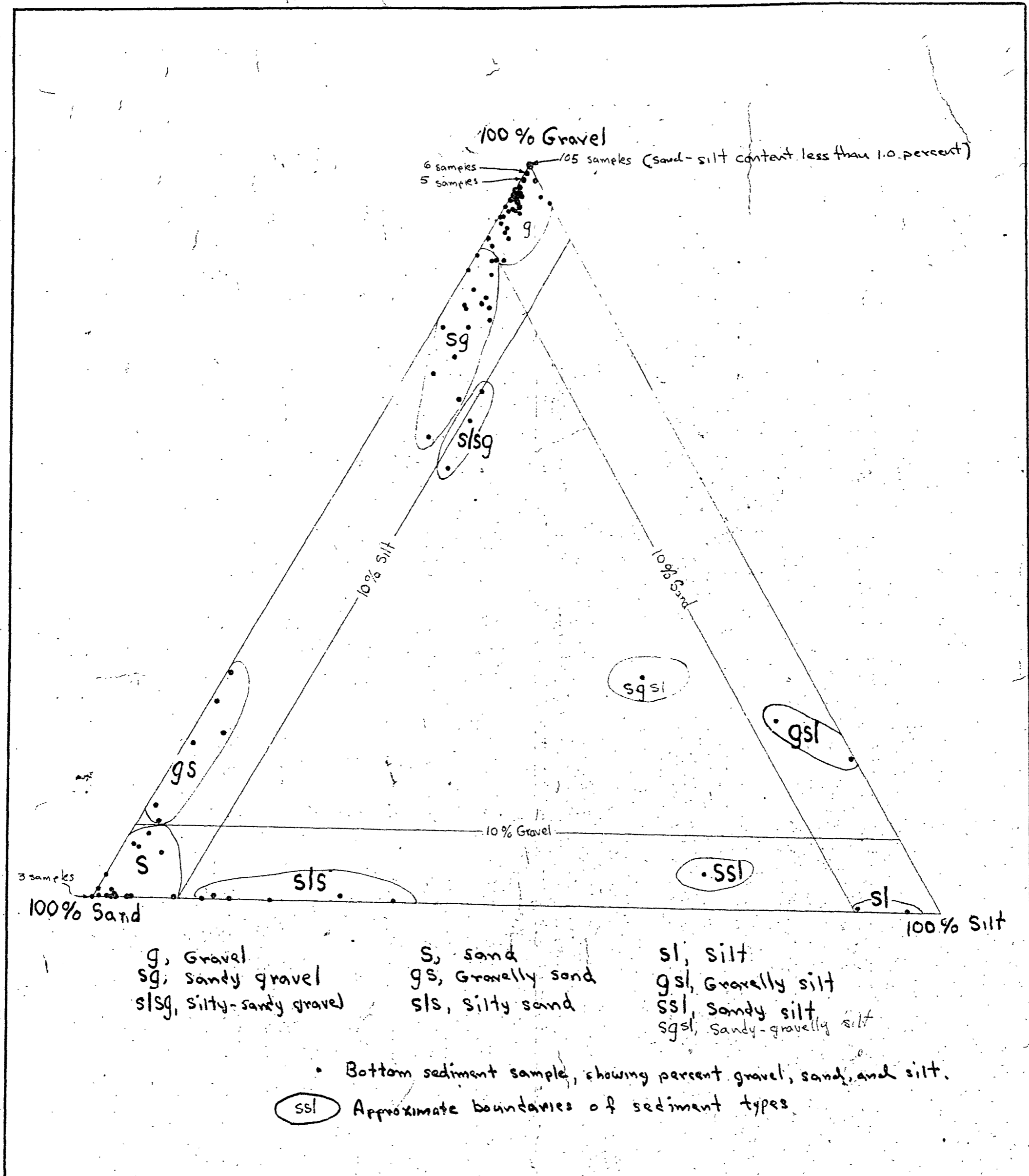
FIGURE 16. Classification of sediment types.
