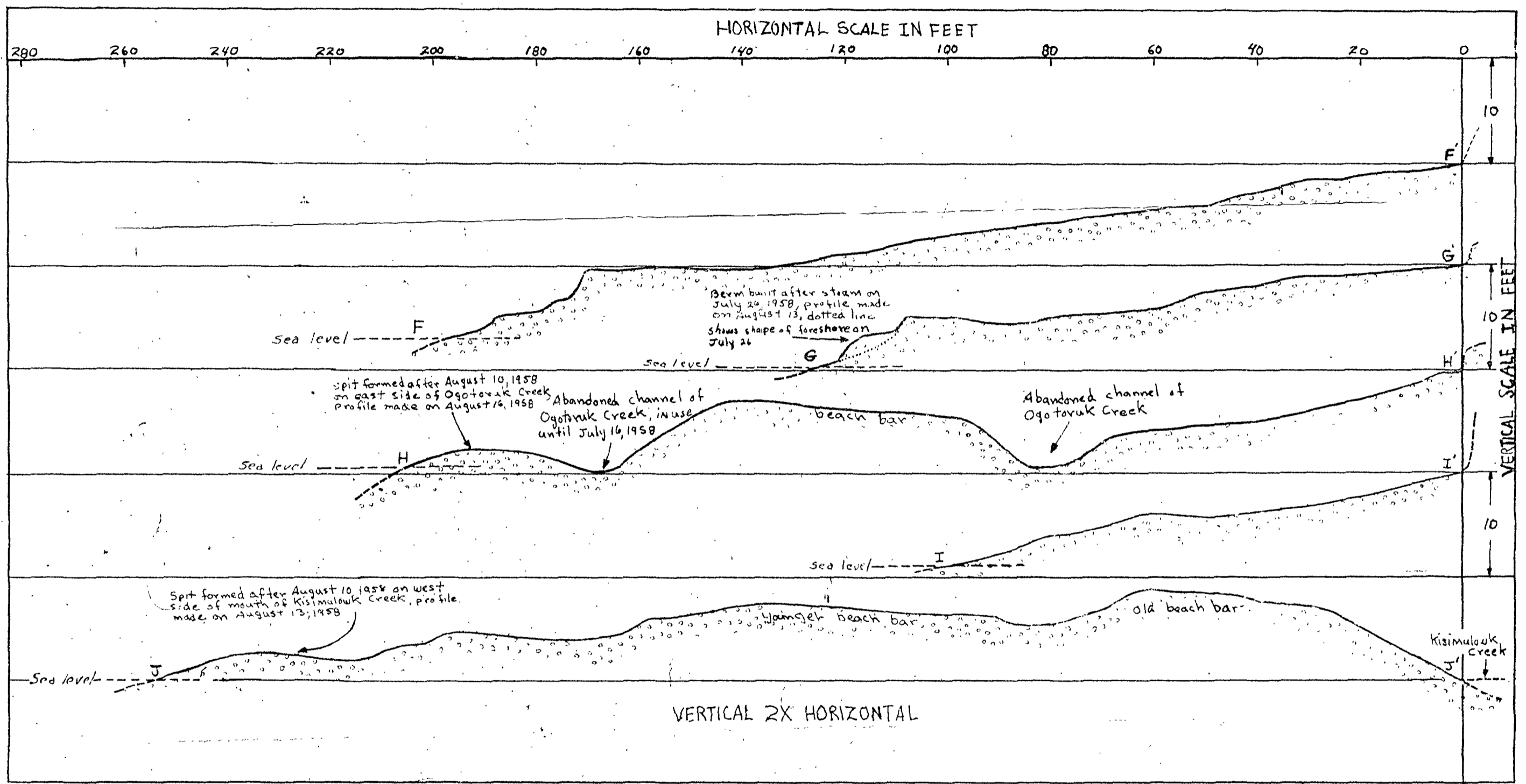
Figure 23. Typical beach profiles, Chukchi Sea, in vicinity of Ogotoruk Creek. See figure 2 for location of profiles
