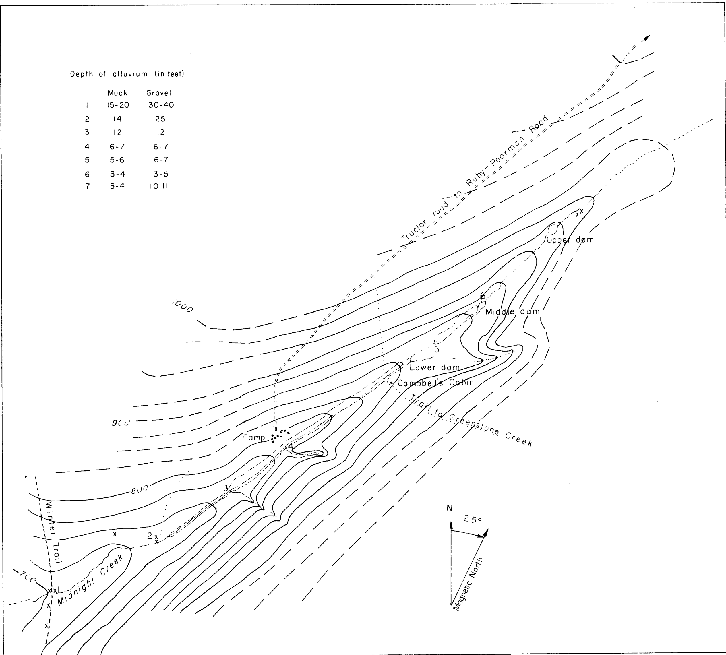
FIGURE 11 - SKETCH MAP OF MINING AREA IN MIDNIGHT CREEK VALLEY SHOWING MINED AREAS AND PROSPECT HOLES
