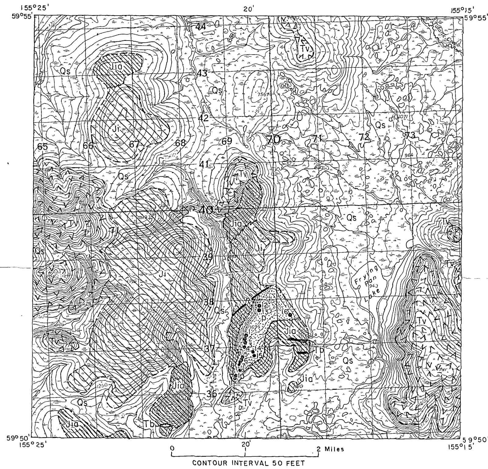
FIGURE 2. Generalized geologic map of part of the Iliamna D-7 quadrangle, Alaska, showing location of magnetite-bearing pyroxenite, and sample locations.
