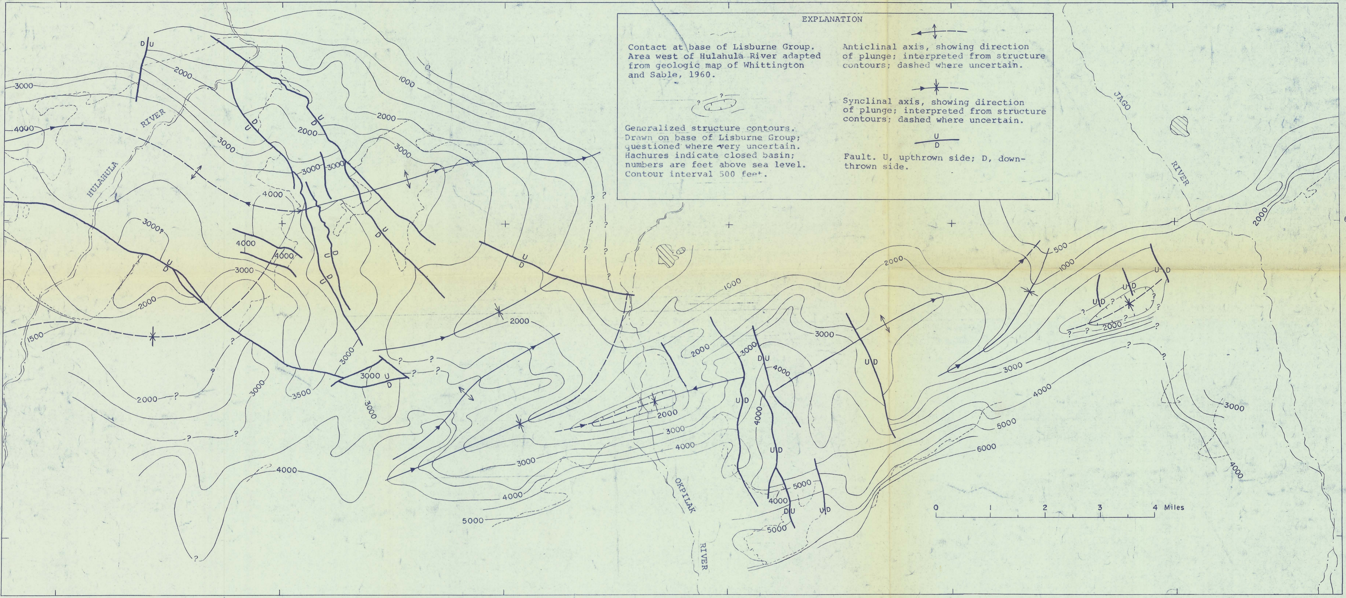
PLATE 3. GENERALIZED STRUCTURE MAP SHOWING BASE OF LISBURNE GROUP, NORTH SIDE OF ROMANZOF MOUNTAINS, ALASKA.
