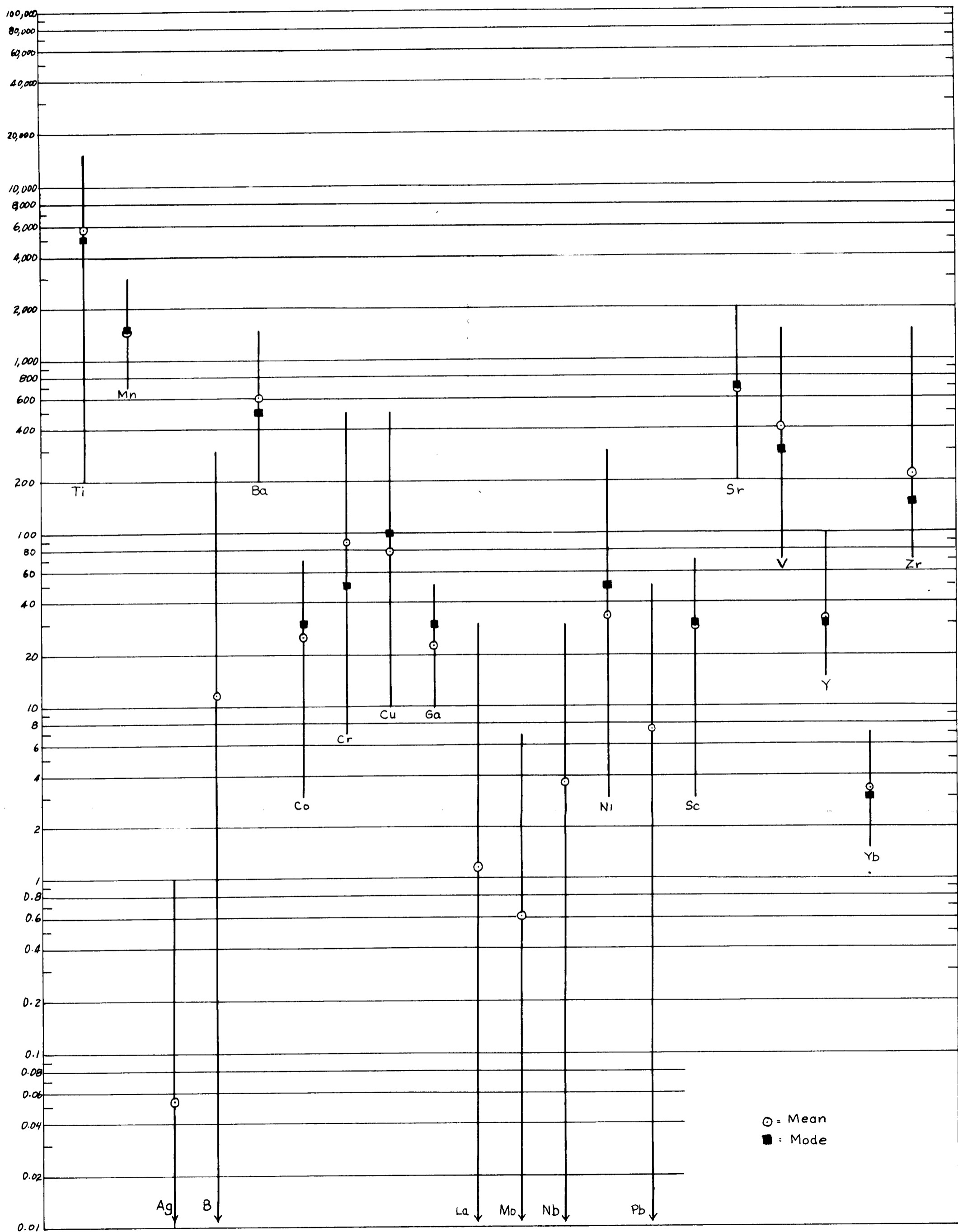
Seven-cycle semi-logarithmic representation of range, mode, and mean for some elements from 127 stream sediment samples in the Hiramna Quadrangle, Alaska. Chart includes samples from this report, and Detterman and Reed (1965, open-file report). Chart does not include pan concentrate of samples 67 and 68 (Detterman and Reed, 1965). Arrows at base of chart denote zero mode. The number of samples in which zero-mode elements were detected is: Ag, 9; B, 52; La, 5; Mo, 11; Nb, 37; Pb, 13.
