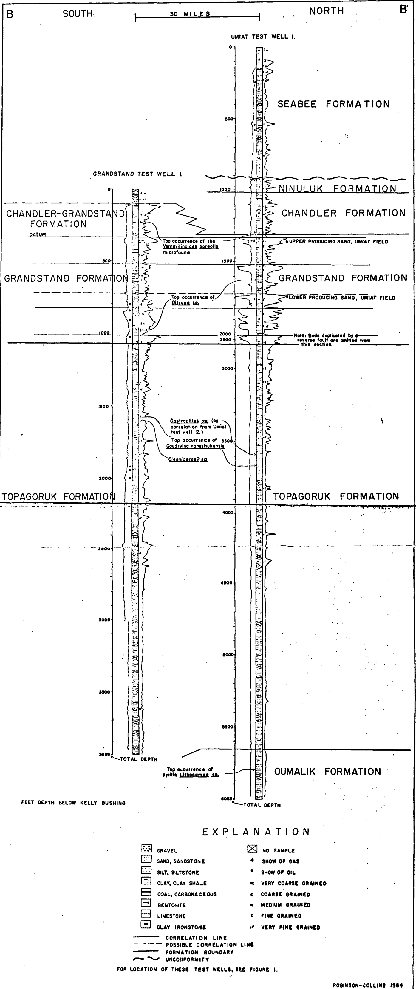
PLATE 2. COMPARISON OF THE SUBSURFACE STRATIGRAPHY IN THE GRANDSTAND AND UMIAT AREAS. ELECTRIC LOG, LITHOLOGIC AND PALEONTOLOGIC CORRELATION OF GRANDSTAND TEST WELL I. AND UMIAT TEST WELL I.
