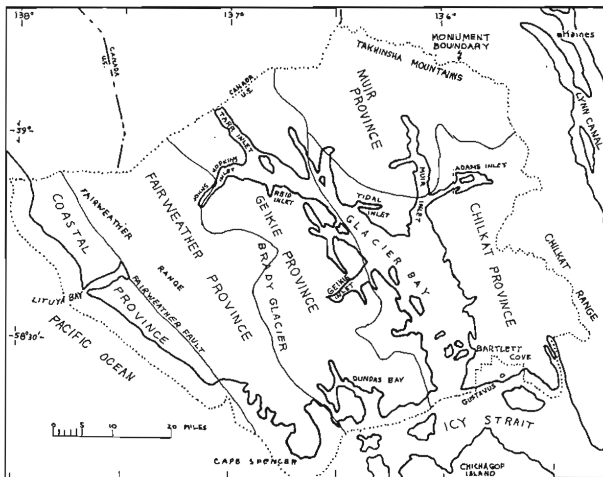
FIGURE 2. INDEX MAP SHOWING GLACIER BAY NATIONAL MONUMENT, ALASKA, GEOLOGIC PROVINCES WITHIN THE MONUMENT, AND LOCALITIES REFERRED TO IN TEXT.
