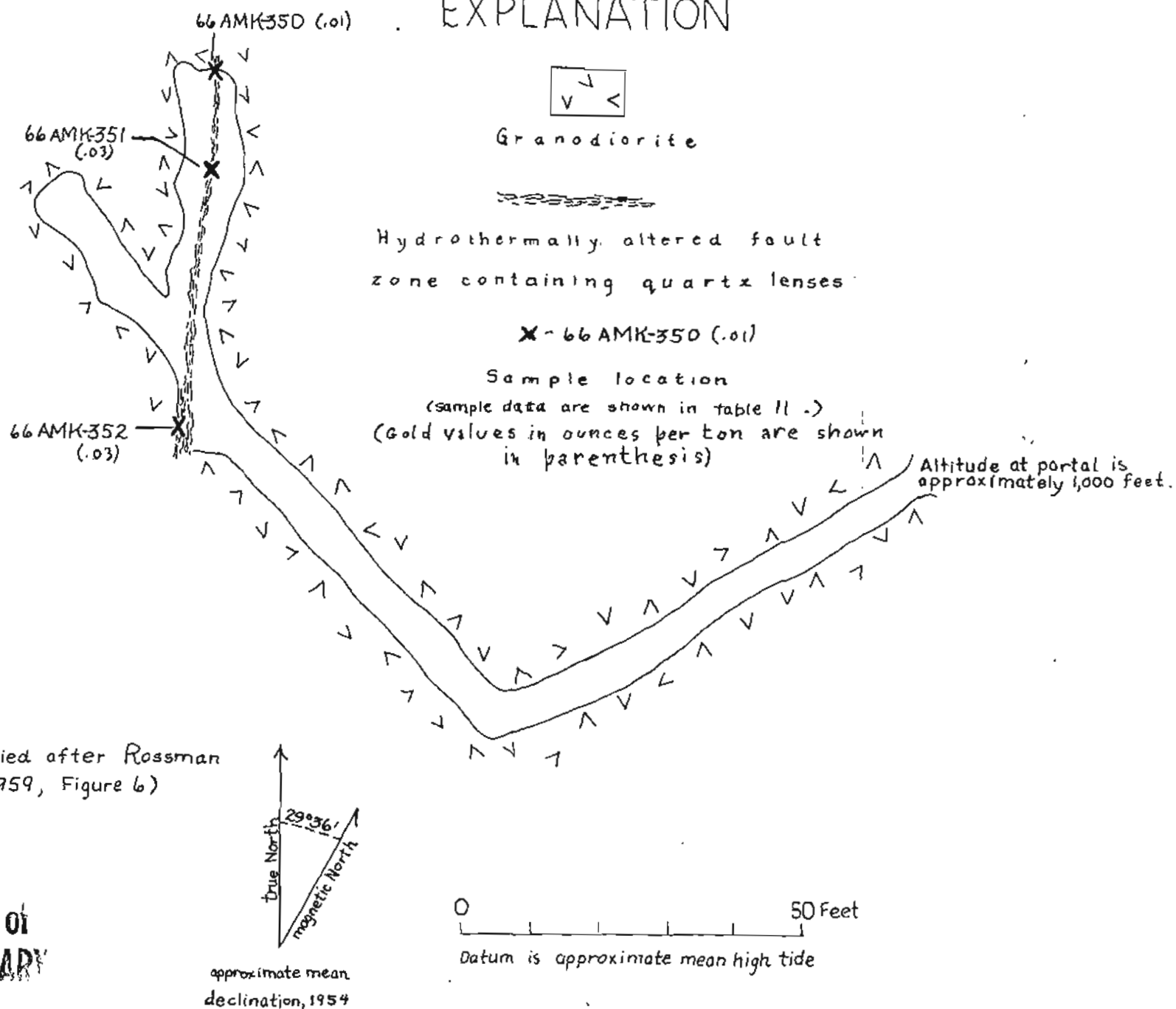
Figure 23. Geologic map and sample locations at the Incas mine.
