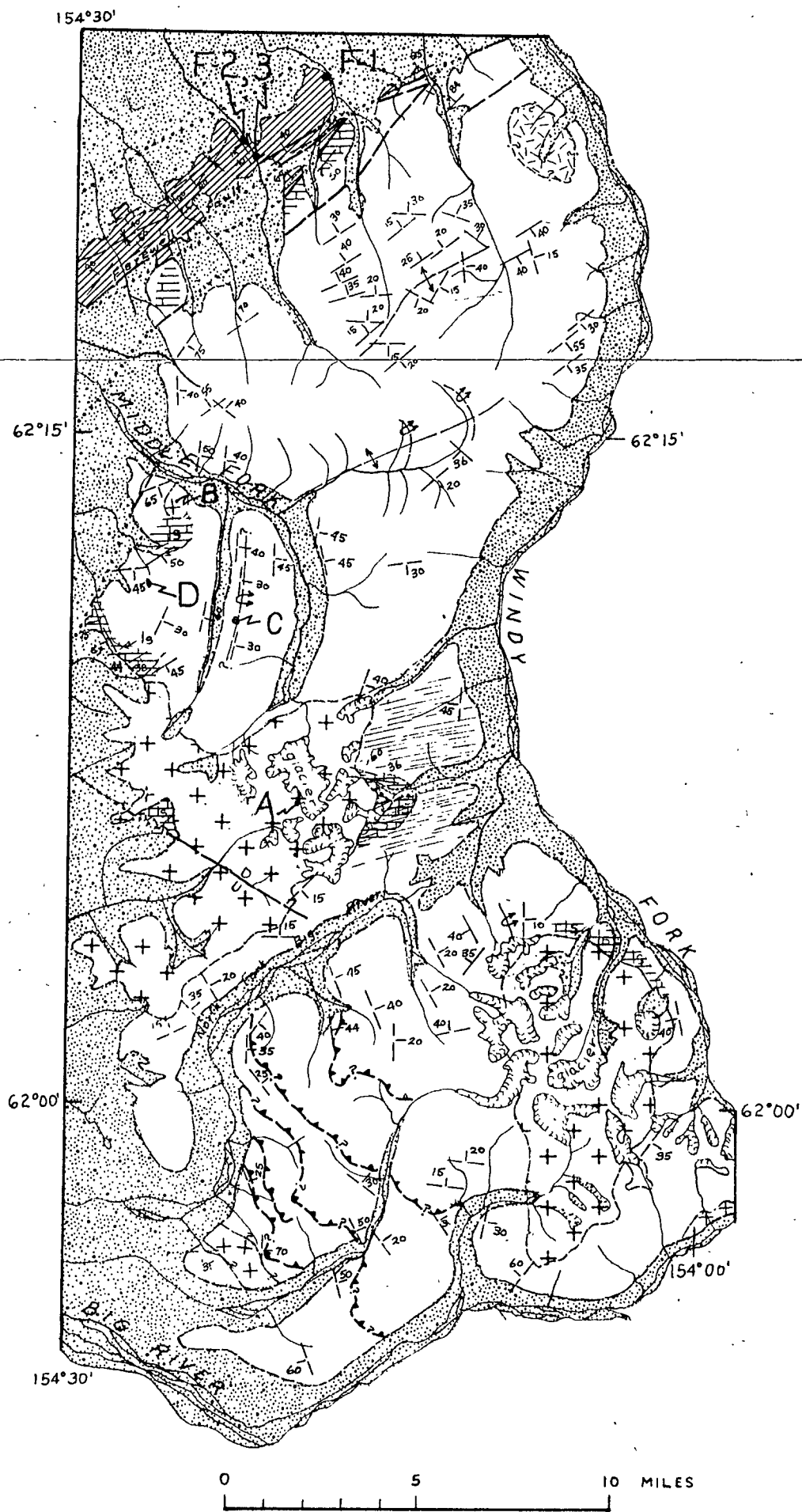
Figure 2. Preliminary geologic reconnaissance of Area I. Letters refer to bedrock localities discussed in text.
