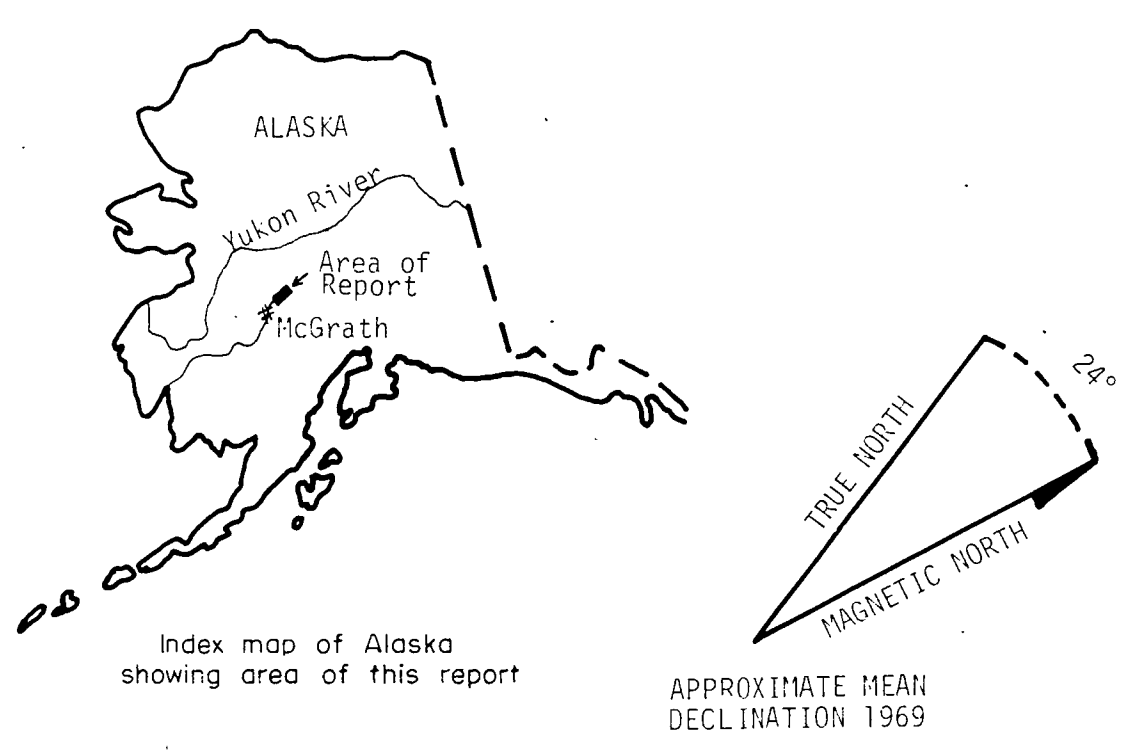
Figure 1.--GEOLOGIC RECONNAISSANCE AND AEROMAGNETIC MAP OF THE NIXON FORK AREA, ALASKA
