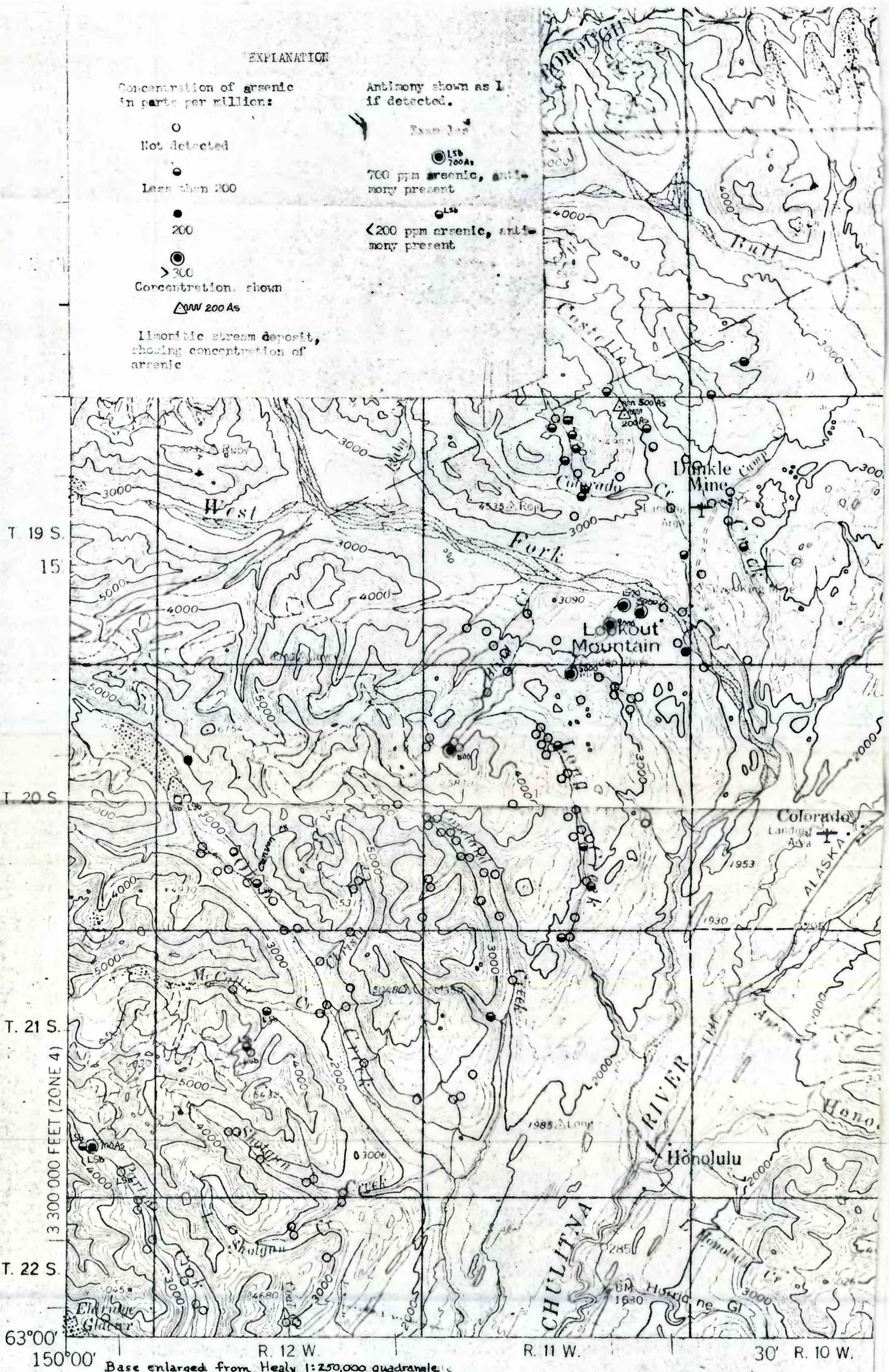
FIGURE 5 -- Arsenic and Antimony concentrations in stream sediment samples.
