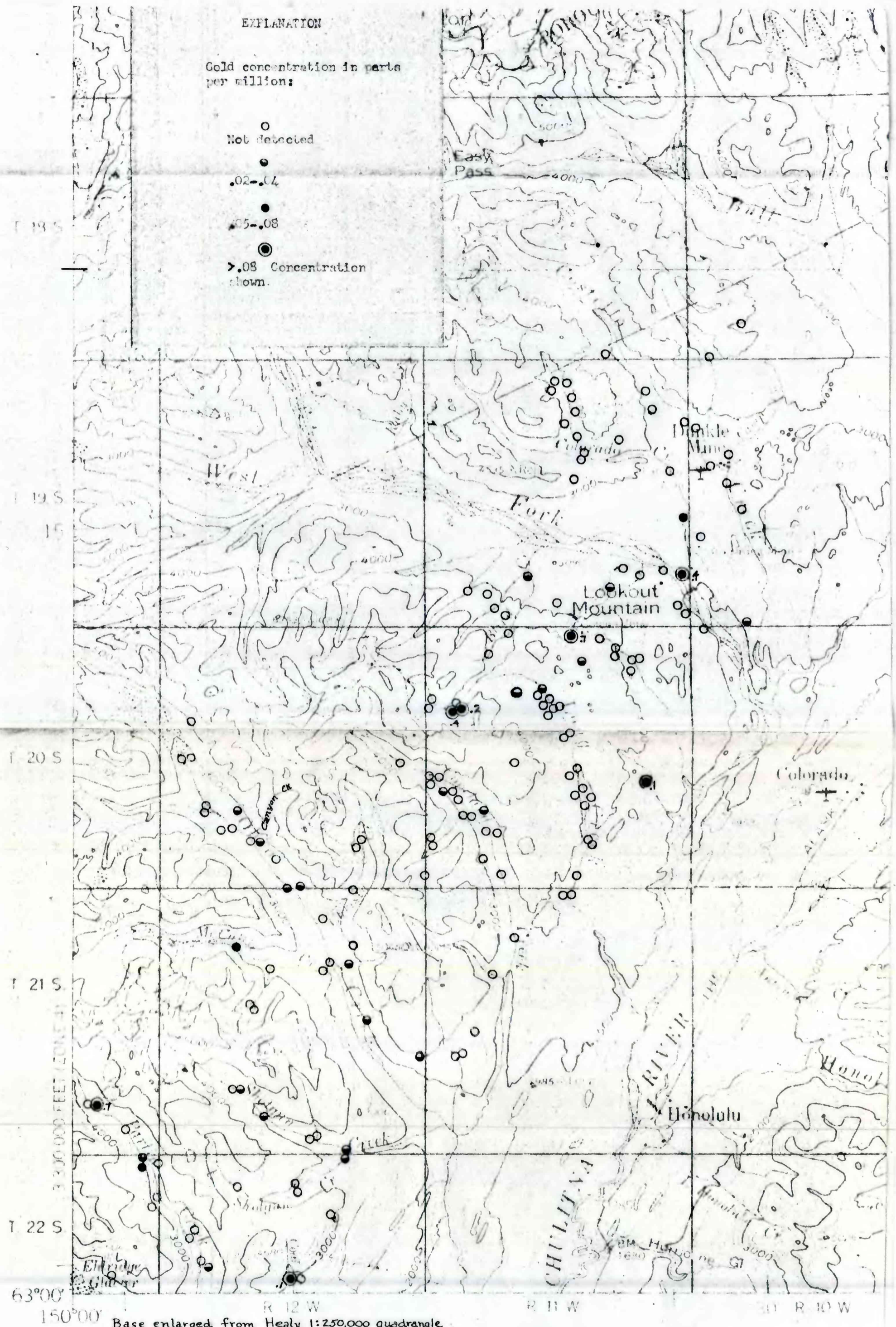
FIGURE 6 -- Gold concentration in stream sediment samples.
