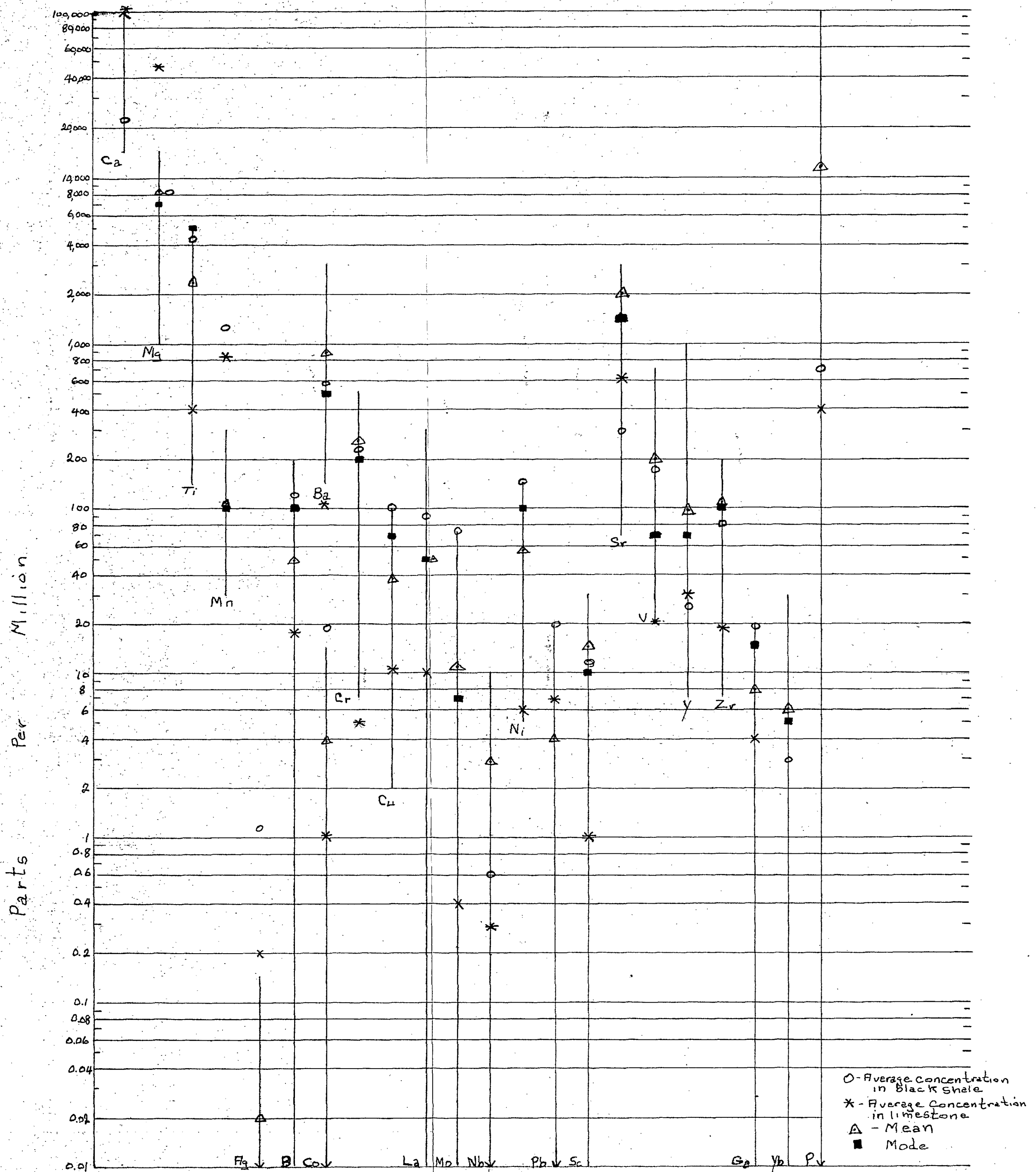
Seven-cycle semi-logarithmic representation of range, mode, and mean for some elements determined by semiquantitative spectrographic analysis on 38 samples from Fire Creek, Mt. Michelson Quadrangle, Alaska. Arrow at base denotes mode zero; arrow at top denotes mode greater than 100,000 ppm. Data for average concentration obtained from Hawkes, E.F. and Webb, J.S., 1962, Geochemistry in Mineral Exploration , and Vinogradov, A.P., 1966, Geochemistry of the Earth's Crust , Vol. 1, pp. 104-118.
