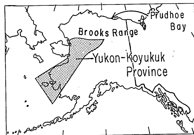
Figure 1. Generalized geologic map of Yukon-Koyukuk Province.
