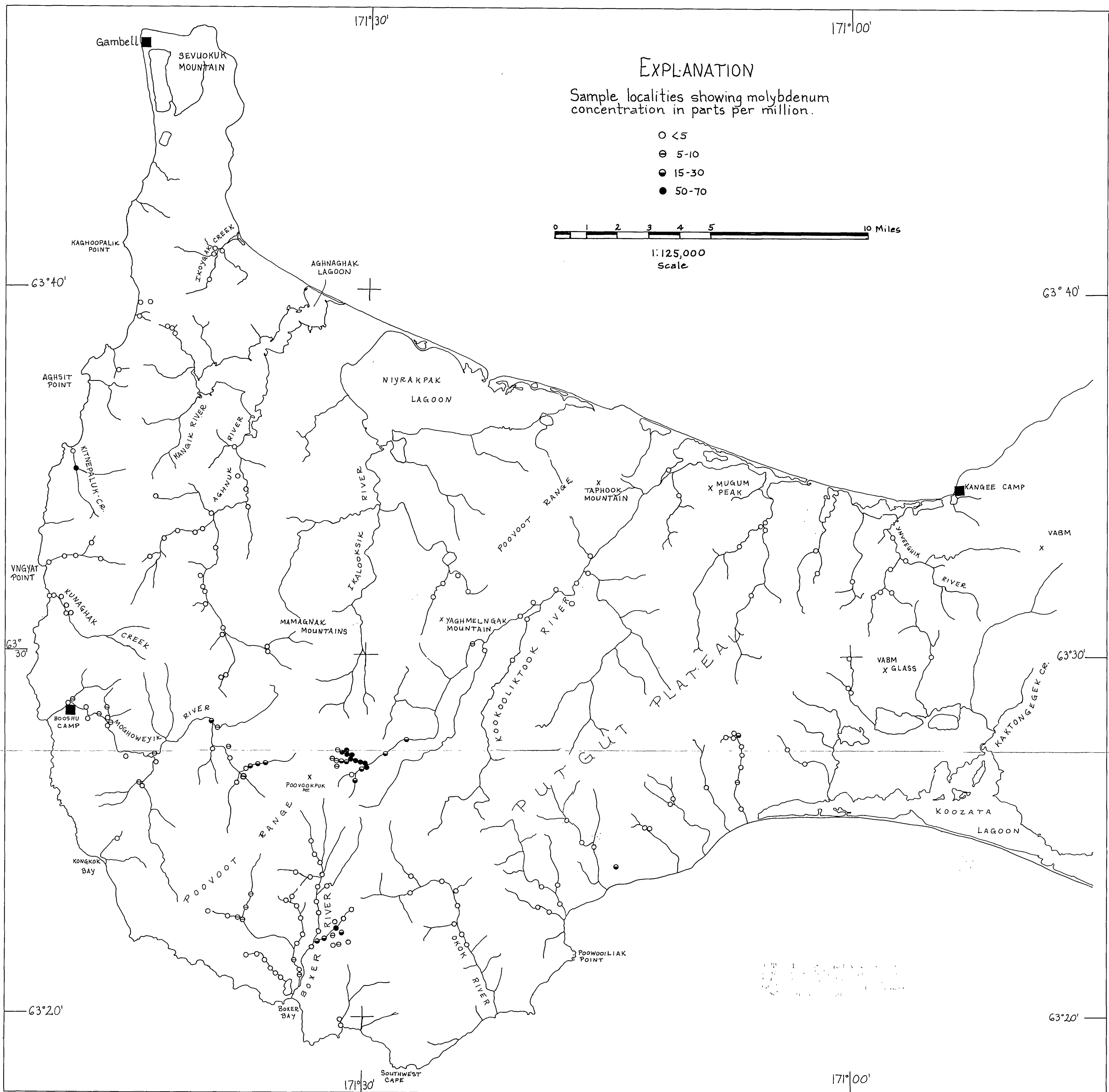
Figure 5. Molybdenum distribution in stream sediment samples of western St. Lawrence Island.
