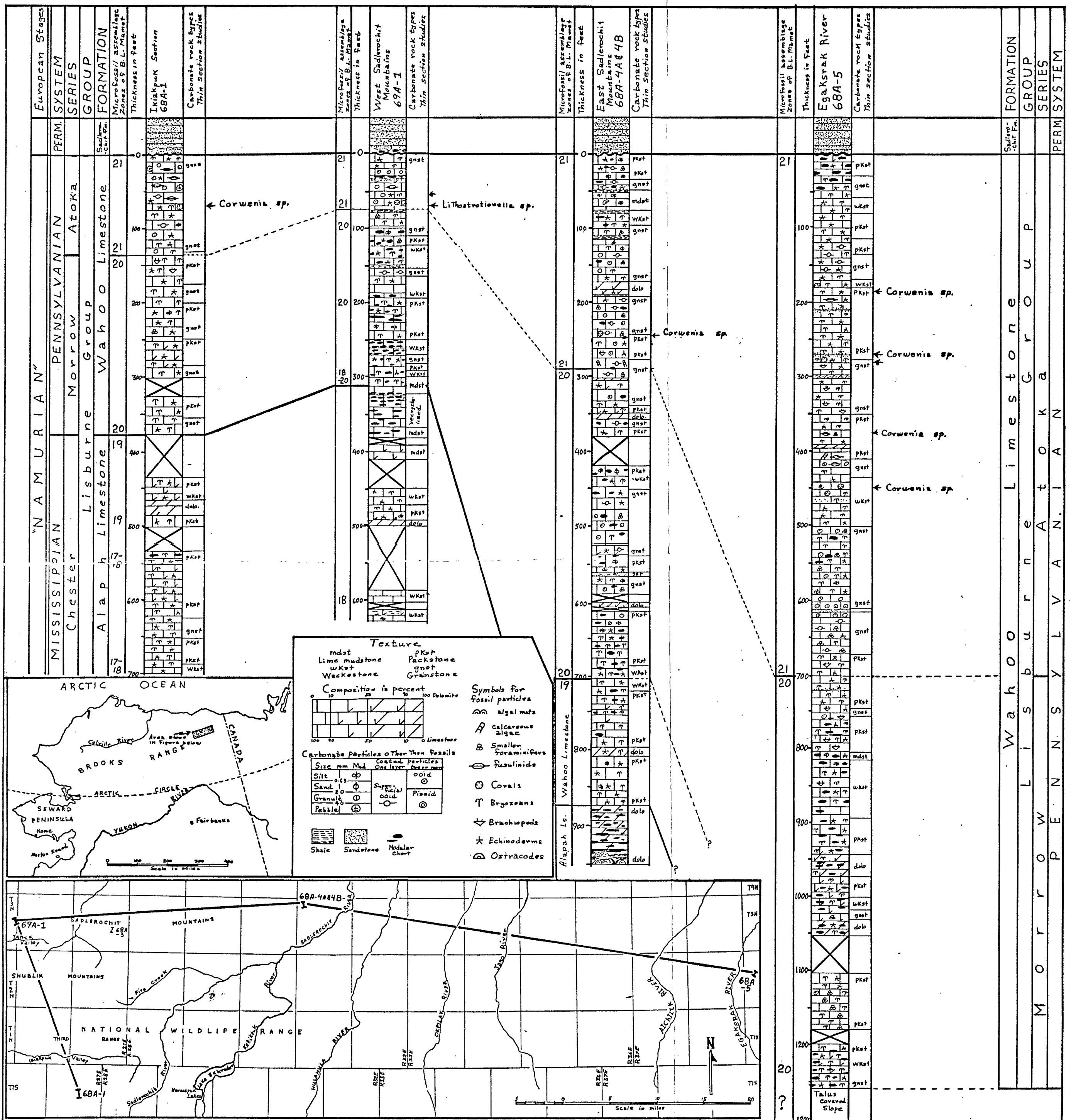
Fig 1 Index map of Arctic Alaska, and a generalised location map of the measured sections of The Wahoo Limestone in northeastern Alaska, with a graphic explanation of The Lithologic and Fossil symbols used in this report. Detailed location maps of the stratigraphic sections given in Figs. 4-9.
