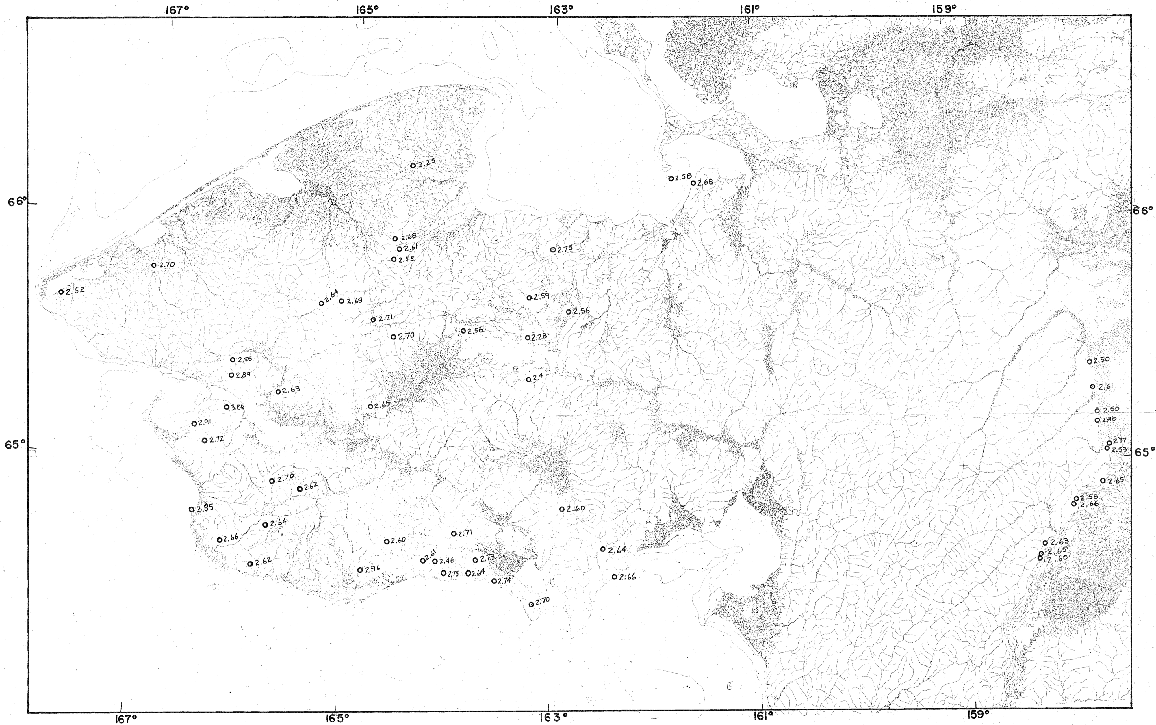
PRELIMINARY MAP 2 OF 4 — SPECIFIC GRAVITY MEASUREMENTS OF ROCK SPECIMENS FROM SEWARD PENINSULA, ALASKA PREPARED BY DAVID F. BARNES U. S. GEOLOGICAL SURVEY FROM DATA DESCRIBED IN SUPPLEMENTARY TEXT
