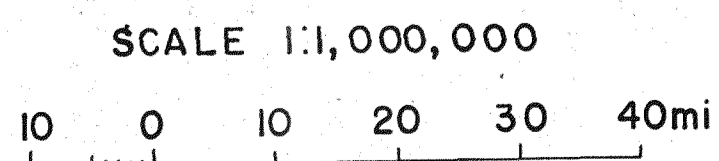
PRELIMINARY MAP 2 OF 4 — SPECIFIC GRAVITY MEASUREMENTS OF ROCK SPECIMENS FROM SEWARD PENINSULA, ALASKA PREPARED BY DAVID F. BARNES U. S. GEOLOGICAL SURVEY FROM DATA DESCRIBED IN SUPPLEMENTARY TEXT
