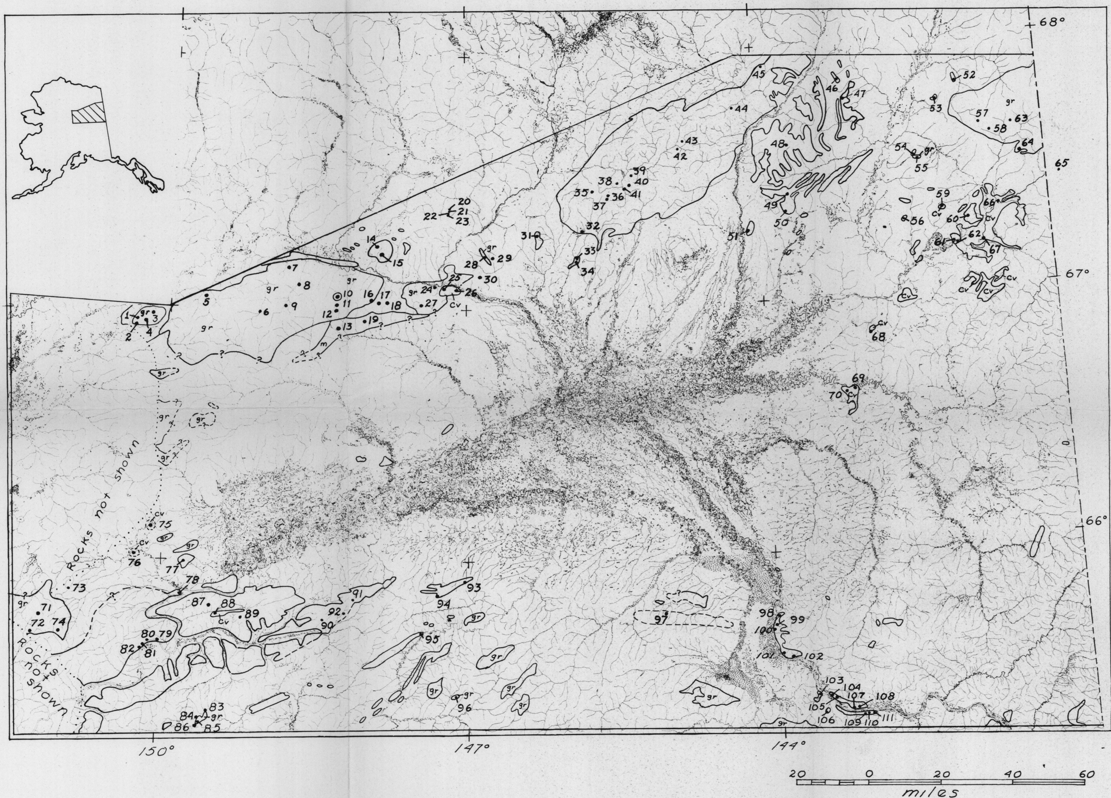
Fig. 1. Yukon River - Porcupine River area, showing location of magnetic susceptibility samples (by map number), and outcrops of granitic rocks (gr), Cenozoic volcanic rocks (Cv), and older mafic and ultramafic rocks (unlabelled outlines).
